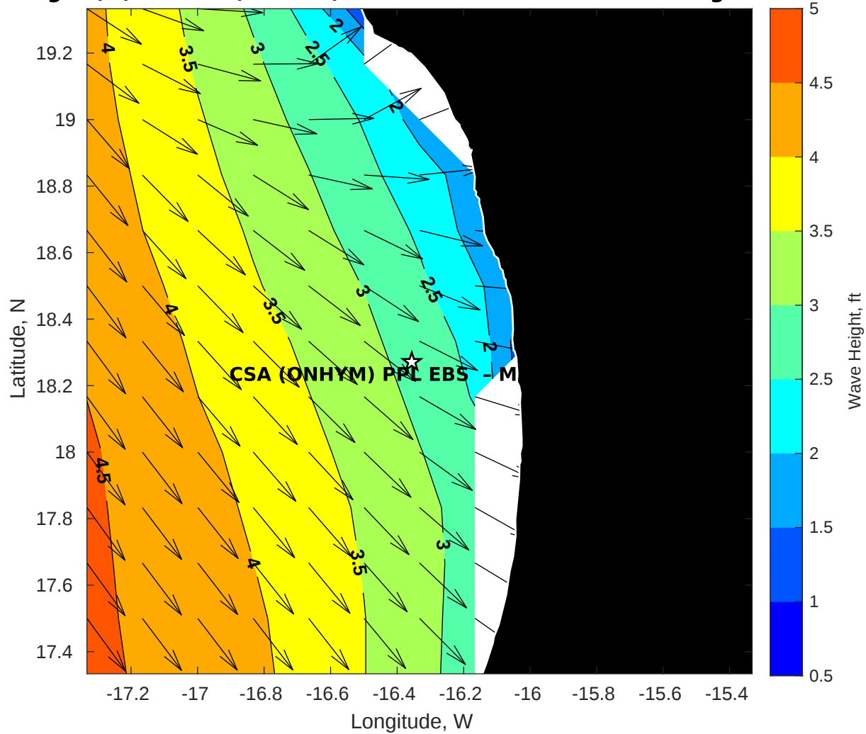
Wave Height (ft) for CSA (ONHYM) PPL EBS - Mauritania at 30-Aug-2025 09:00:00
