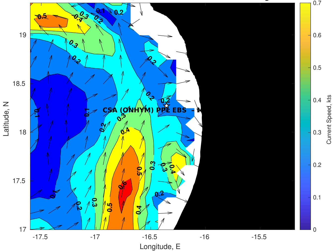
Surface Currents for CSA (ONHYM) PPL EBS - Mauritania at 29-Aug-2025 00:00:00
