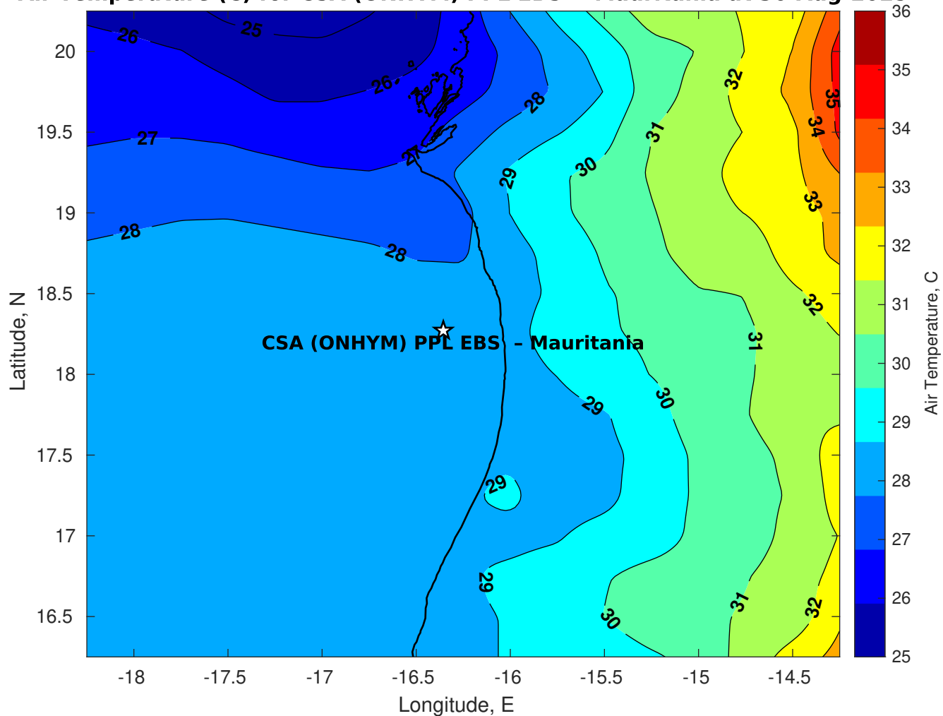
Air Temperature (C) for CSA (ONHYM) PPL EBS - Mauritania at 30-Aug-2025
