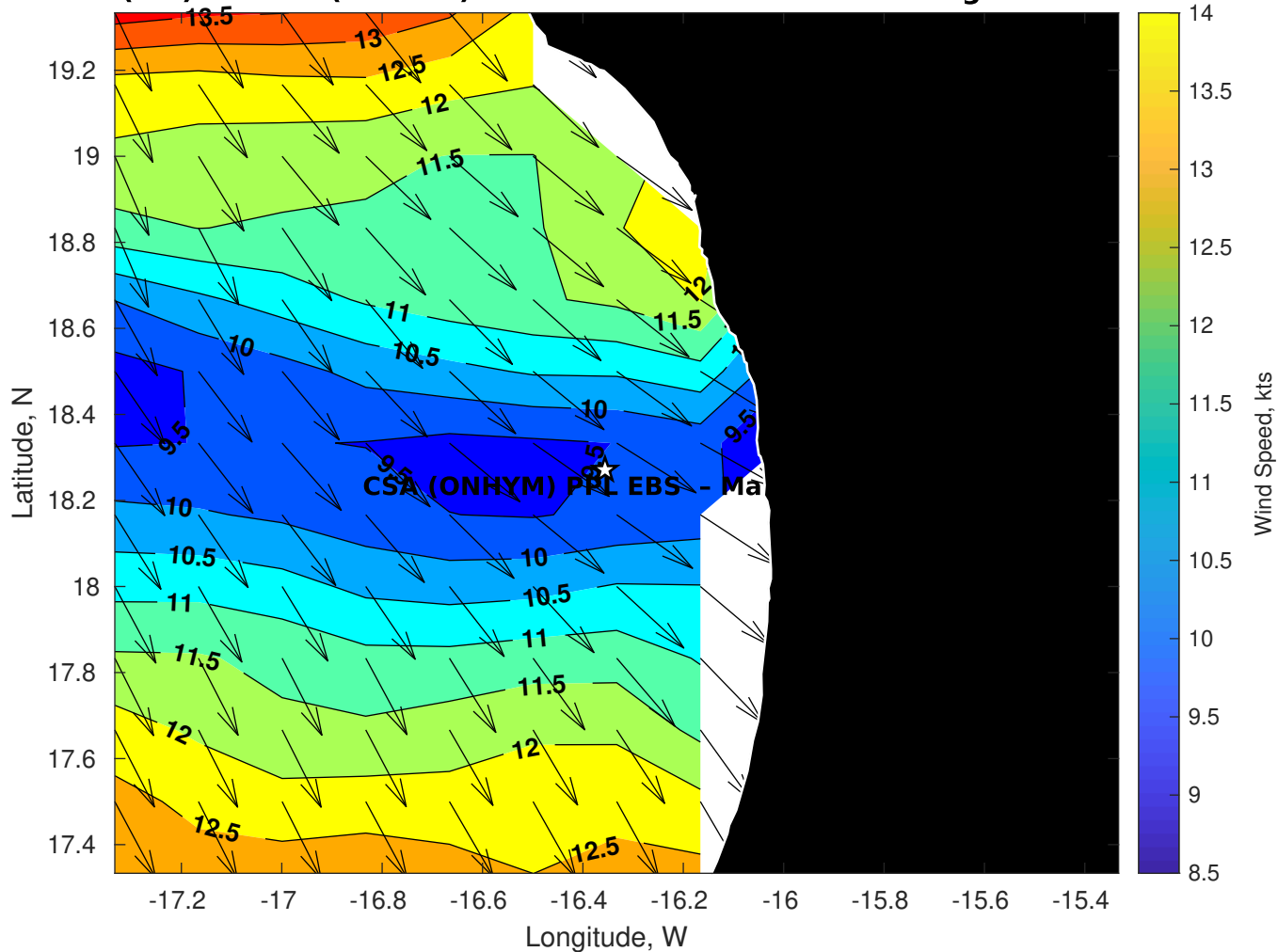
Winds (kts) for CSA (ONHYM) PPL EBS - Mauritania at 30-Aug-2025 09:00:00
