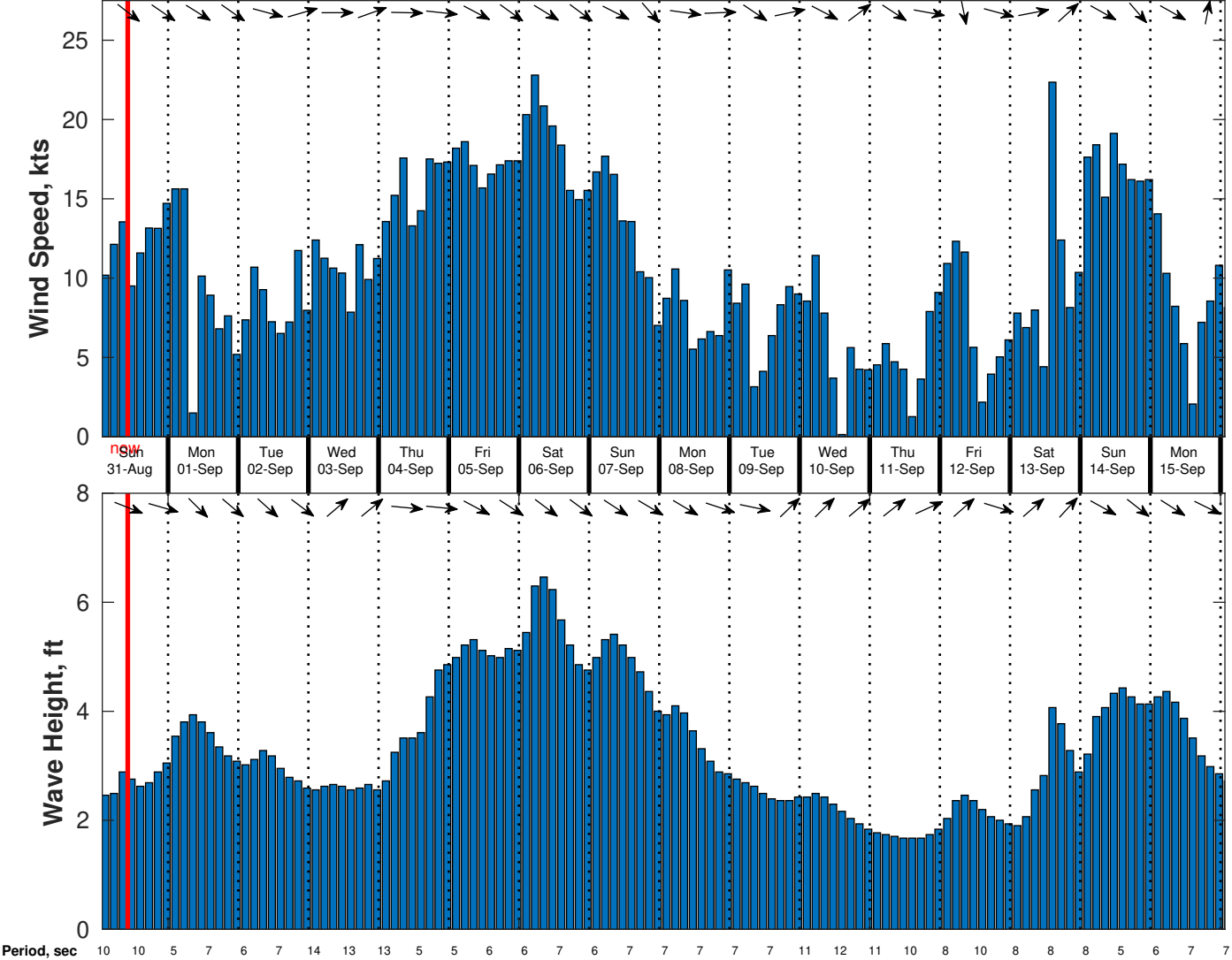
Wind & Wave Forecast for CSA (ONHYM) PPL EBS - Mauritania from 30-Aug-2025 01:00:00 to 15-Sep-2025 01:00:00
