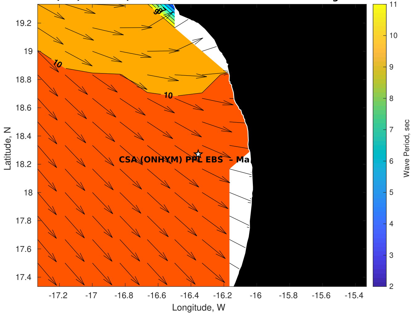
Wave Period (sec) for CSA (ONHYM) PPL EBS - Mauritania at 30-Aug-2025 09:00:00
