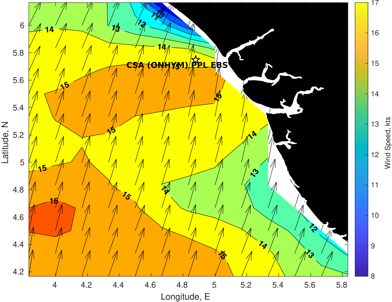
Winds (kts) for CSA (ONHYM) PPL EBS - Nigeria at 30-Aug-2025 09:00:00
