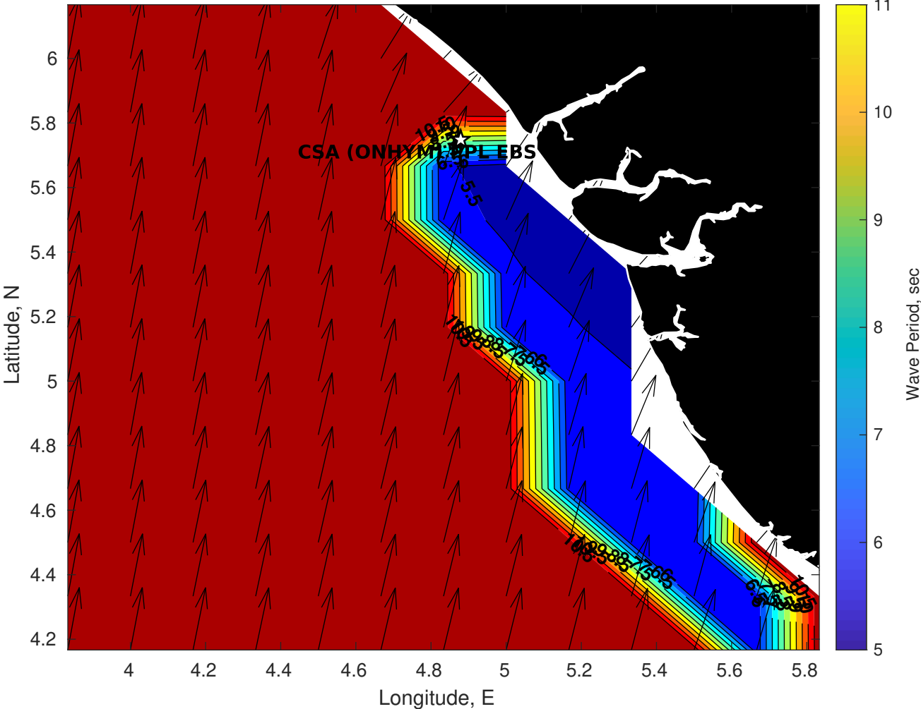
Wave Period (sec) for CSA (ONHYM) PPL EBS - Nigeria at 30-Aug-2025 09:00:00
