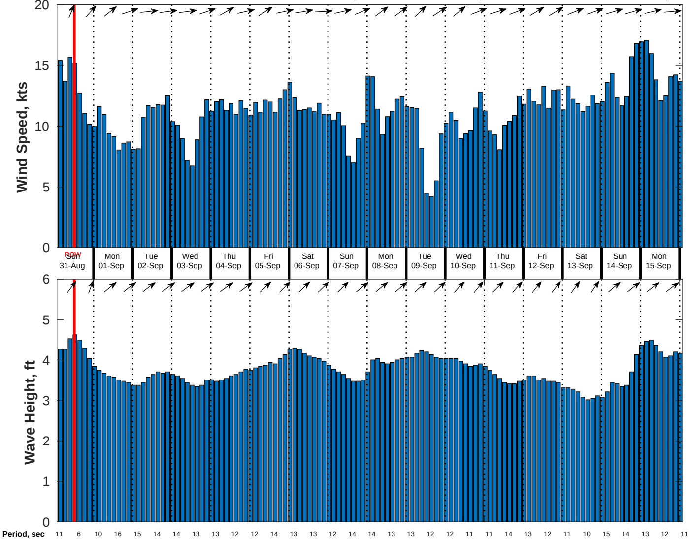
Wind & Wave Forecast for CSA (ONHYM) PPL EBS - Nigeria from 30-Aug-2025 02:00:00 to 15-Sep-2025 02:00:00
