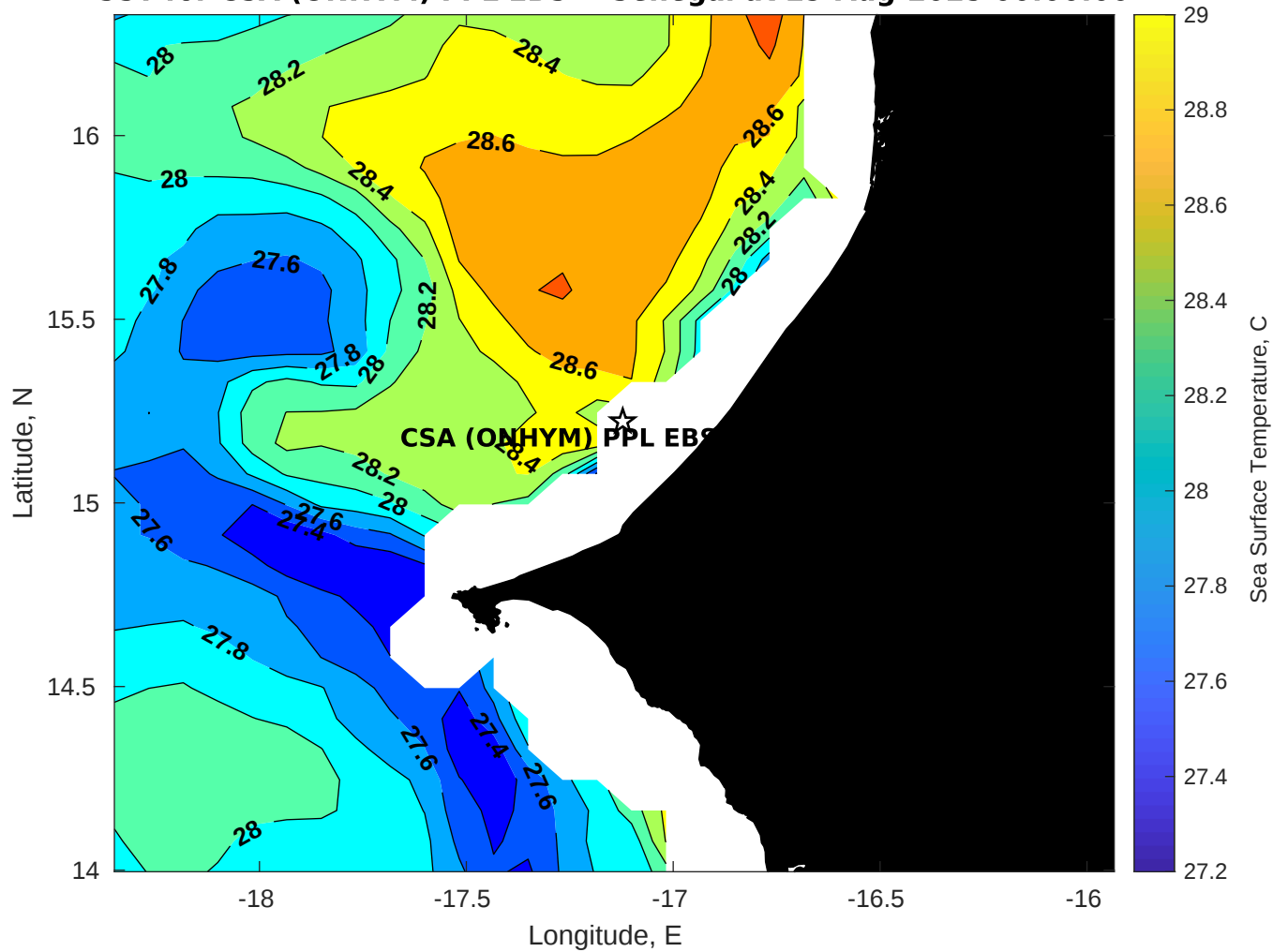
SST for CSA (ONHYM) PPL EBS - Senegal at 29-Aug-2025 00:00:00
