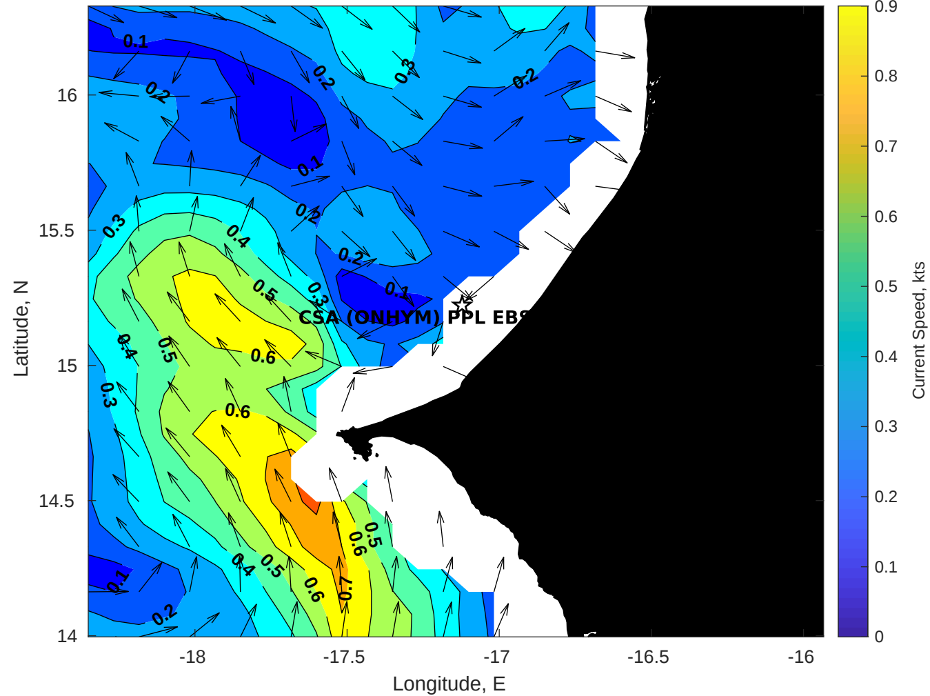
Surface Currents for CSA (ONHYM) PPL EBS - Senegal at 29-Aug-2025 00:00:00
