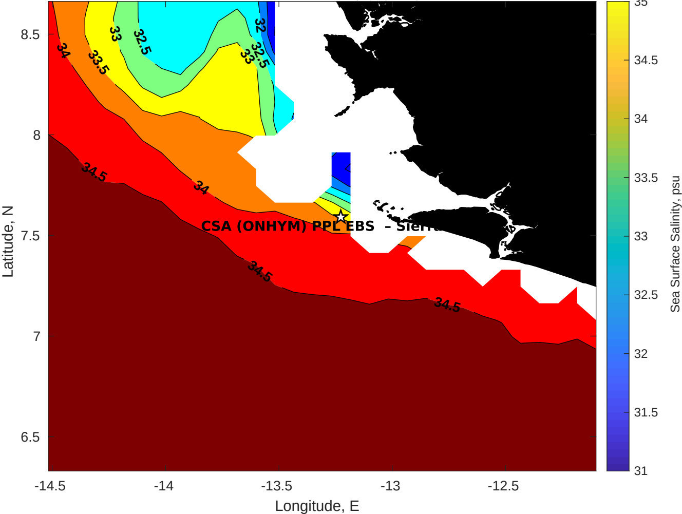
Surface Salinity for CSA (ONHYM) PPL EBS - Sierra Leone at 29-Aug-2025 00:00:00
