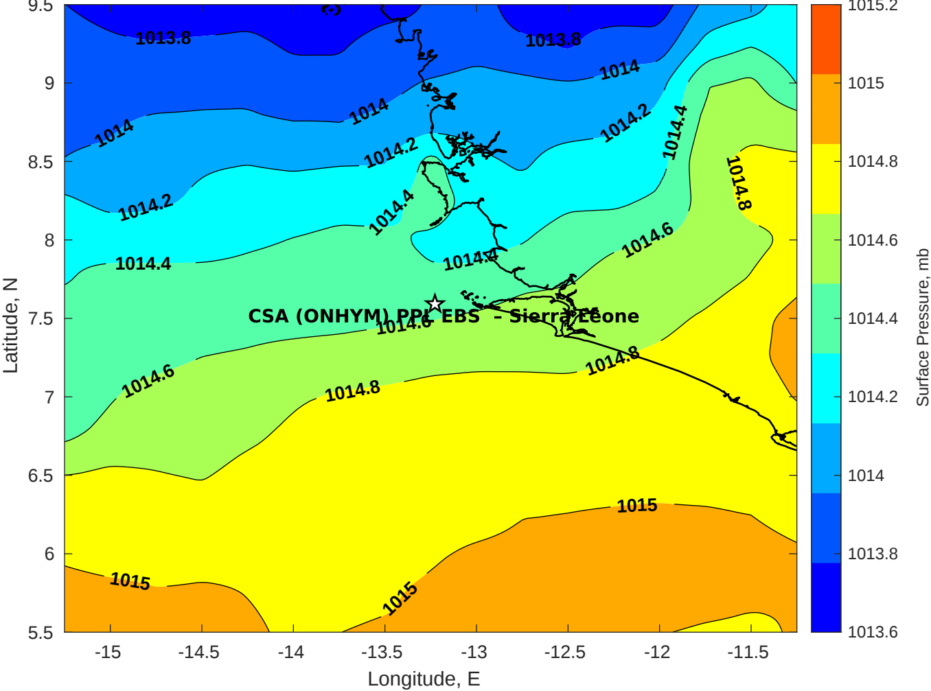
Surface Pressure (mb) for CSA (ONHYM) PPL EBS - Sierra Leone at 31-Aug-2025 00:00:00
