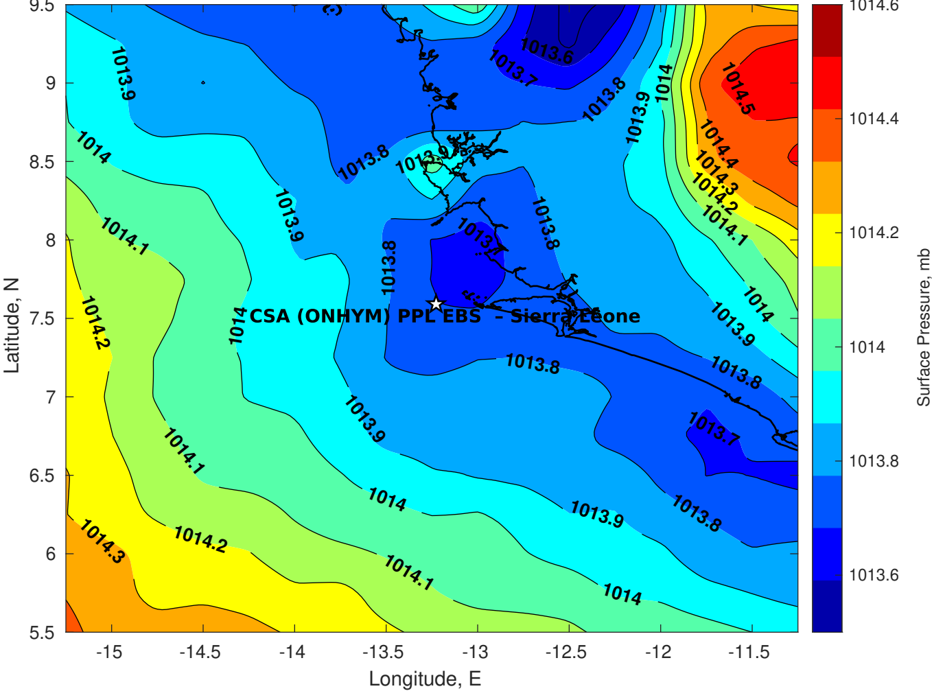
Surface Pressure (mb) for CSA (ONHYM) PPL EBS - Sierra Leone at 30-Aug-2025 00:00:00
