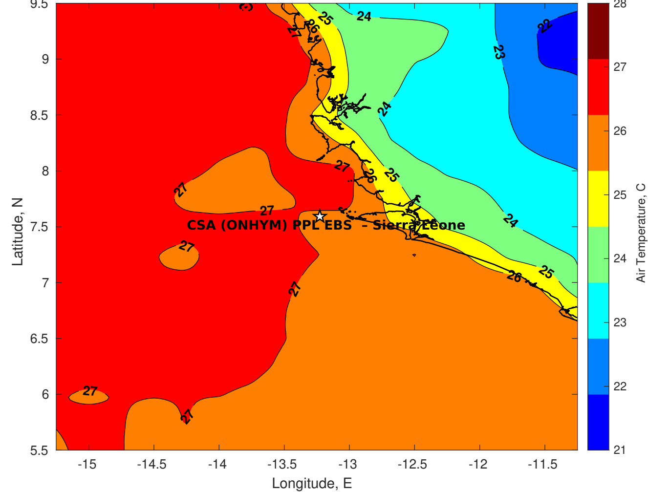
Air Temperature (C) for CSA (ONHYM) PPL EBS - Sierra Leone at 30-Aug-2025
