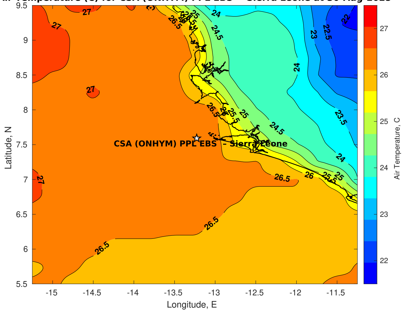
Air Temperature (C) for CSA (ONHYM) PPL EBS - Sierra Leone at 30-Aug-2025
