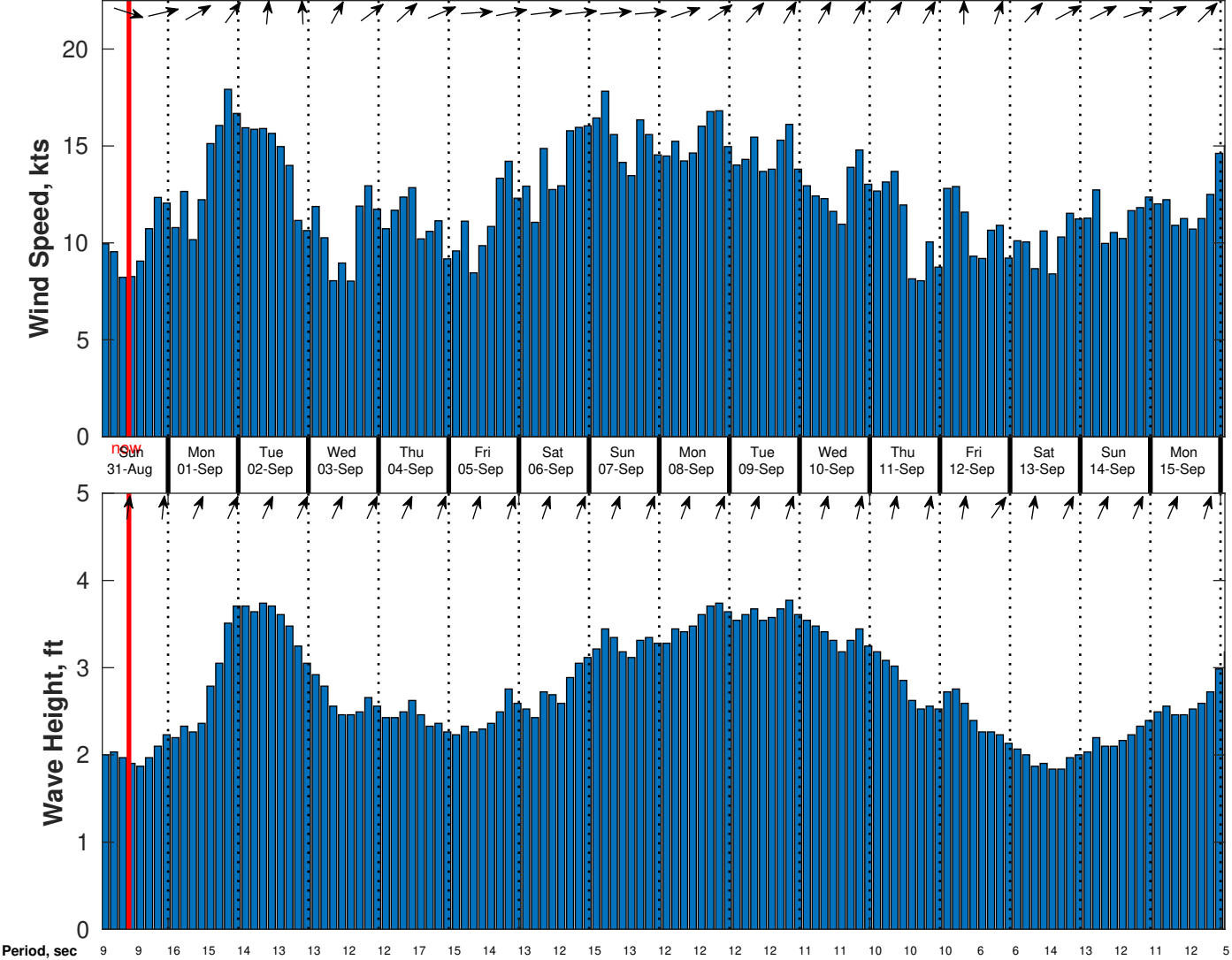
Wind & Wave Forecast for CSA (ONHYM) PPL EBS - Sierra Leone from 30-Aug-2025 01:00:00 to 15-Sep-2025 01:00:00
