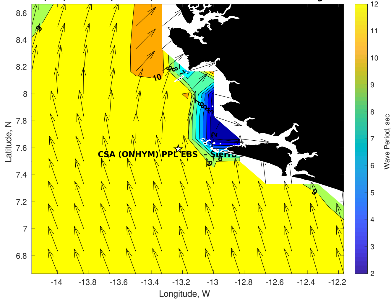
Wave Period (sec) for CSA (ONHYM) PPL EBS - Sierra Leone at 30-Aug-2025 09:00:00
