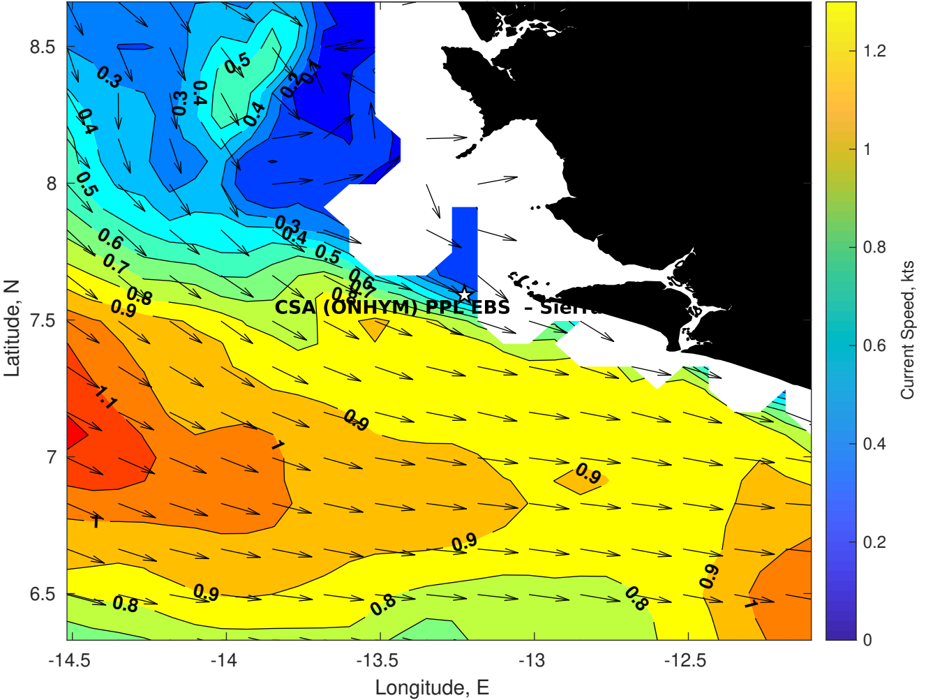
Surface Currents for CSA (ONHYM) PPL EBS - Sierra Leone at 29-Aug-2025 00:00:00
