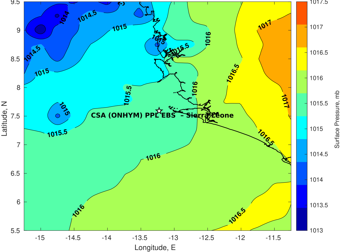
Surface Pressure (mb) for CSA (ONHYM) PPL EBS - Sierra Leone at 01-Sep-2025 00:00:00
