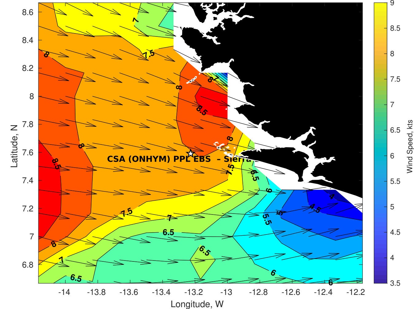
Winds (kts) for CSA (ONHYM) PPL EBS - Sierra Leone at 30-Aug-2025 09:00:00
