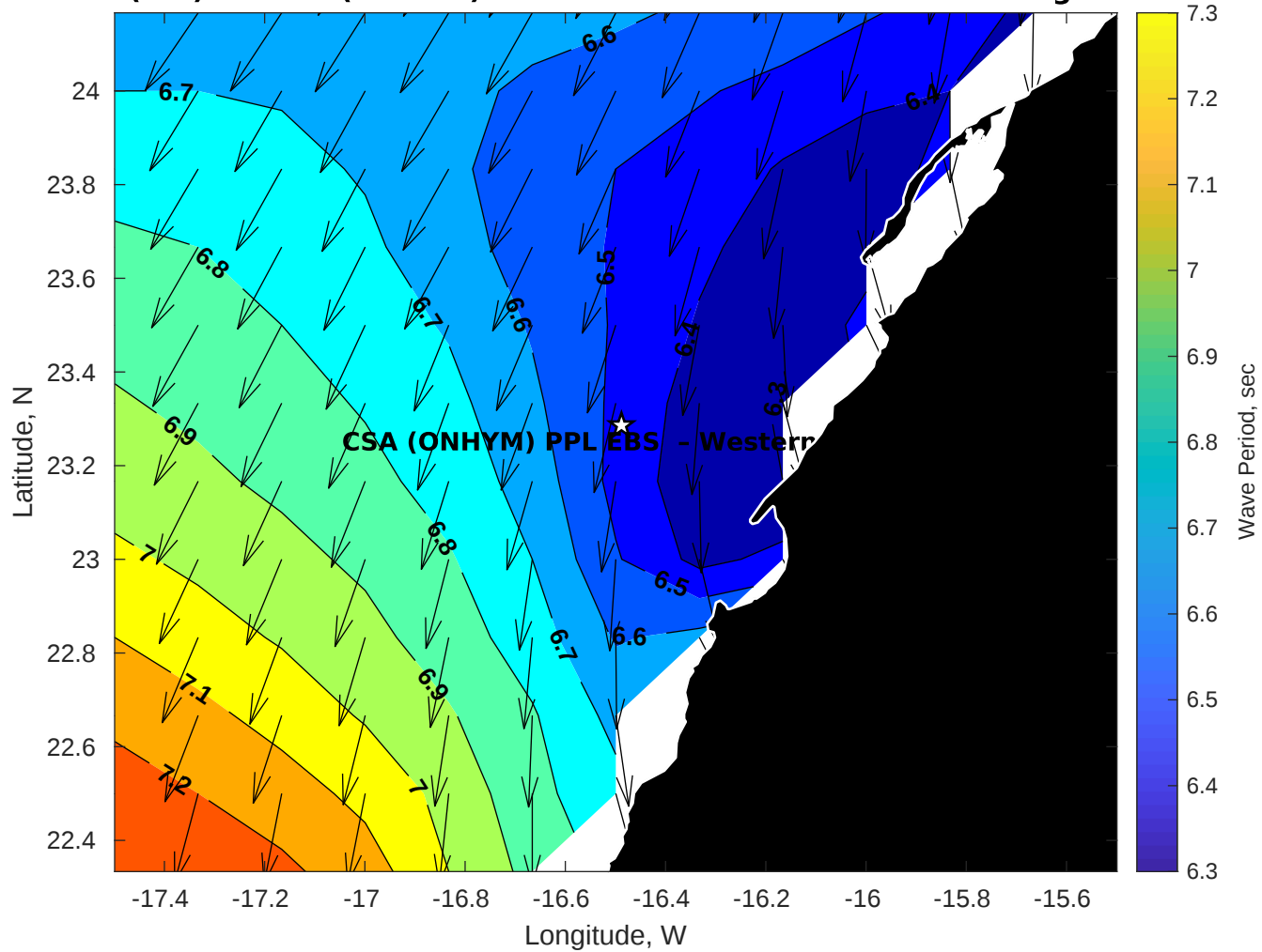
Wave Period (sec) for CSA (ONHYM) PPL EBS - Western Sahara at 30-Aug-2025 09:00:00
