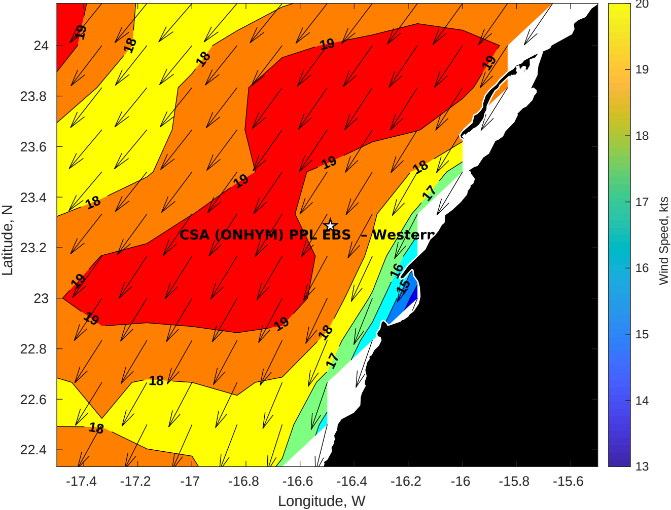
Winds (kts) for CSA (ONHYM) PPL EBS - Western Sahara at 30-Aug-2025 09:00:00
