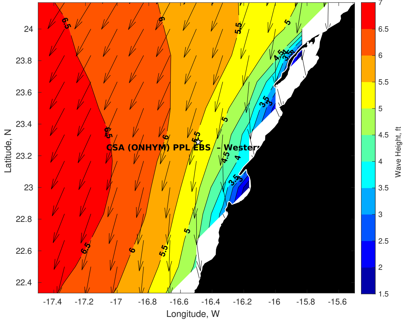
Wave Height (ft) for CSA (ONHYM) PPL EBS - Western Sahara at 30-Aug-2025 09:00:00
