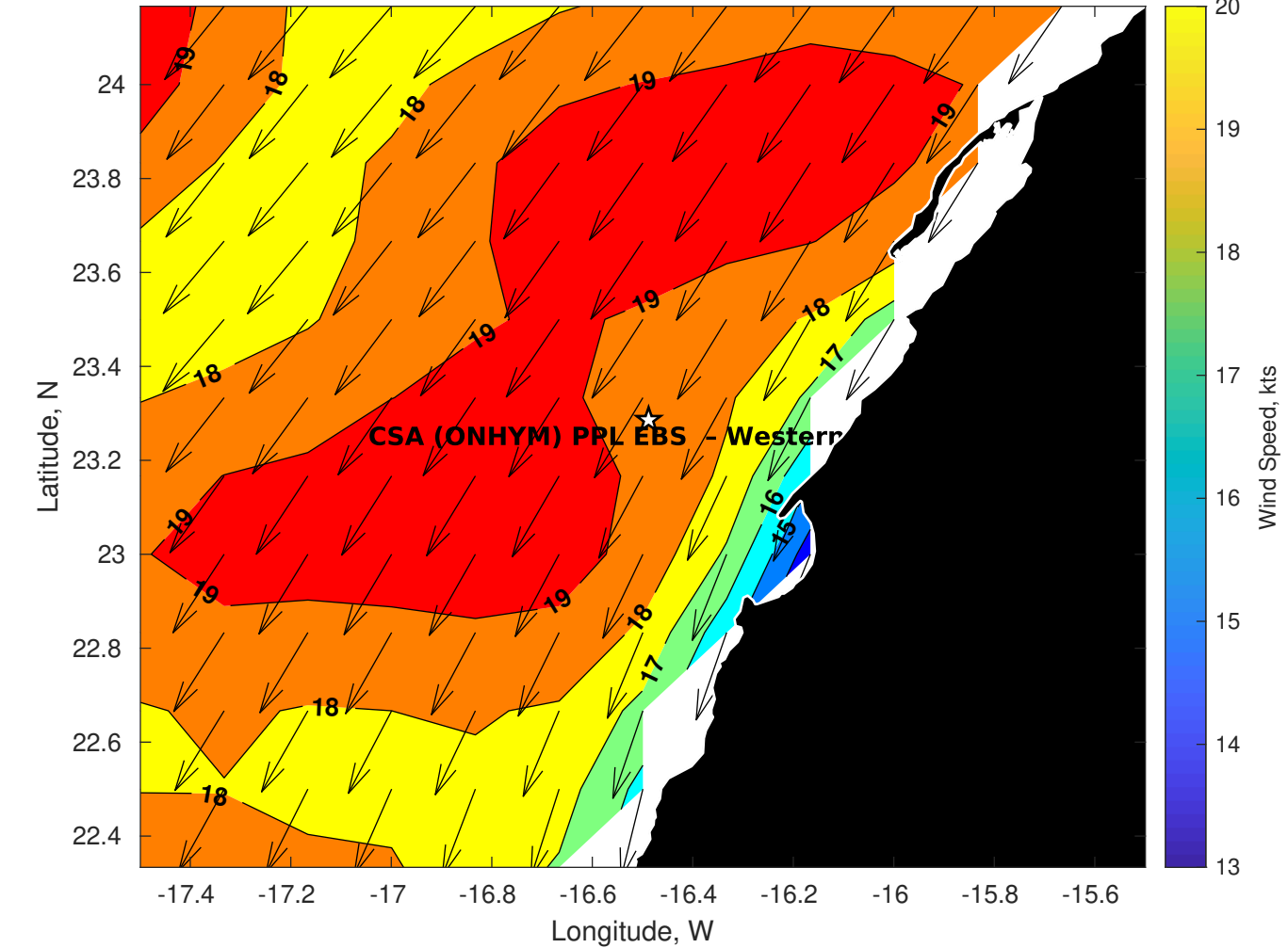
Winds (kts) for CSA (ONHYM) PPL EBS - Western Sahara at 30-Aug-2025 09:00:00
