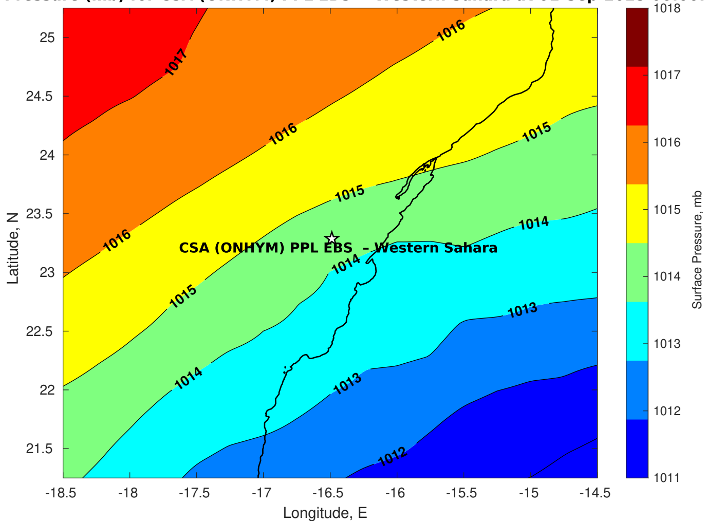
Surface Pressure (mb) for CSA (ONHYM) PPL EBS - Western Sahara at 01-Sep-2025 00:00:00
