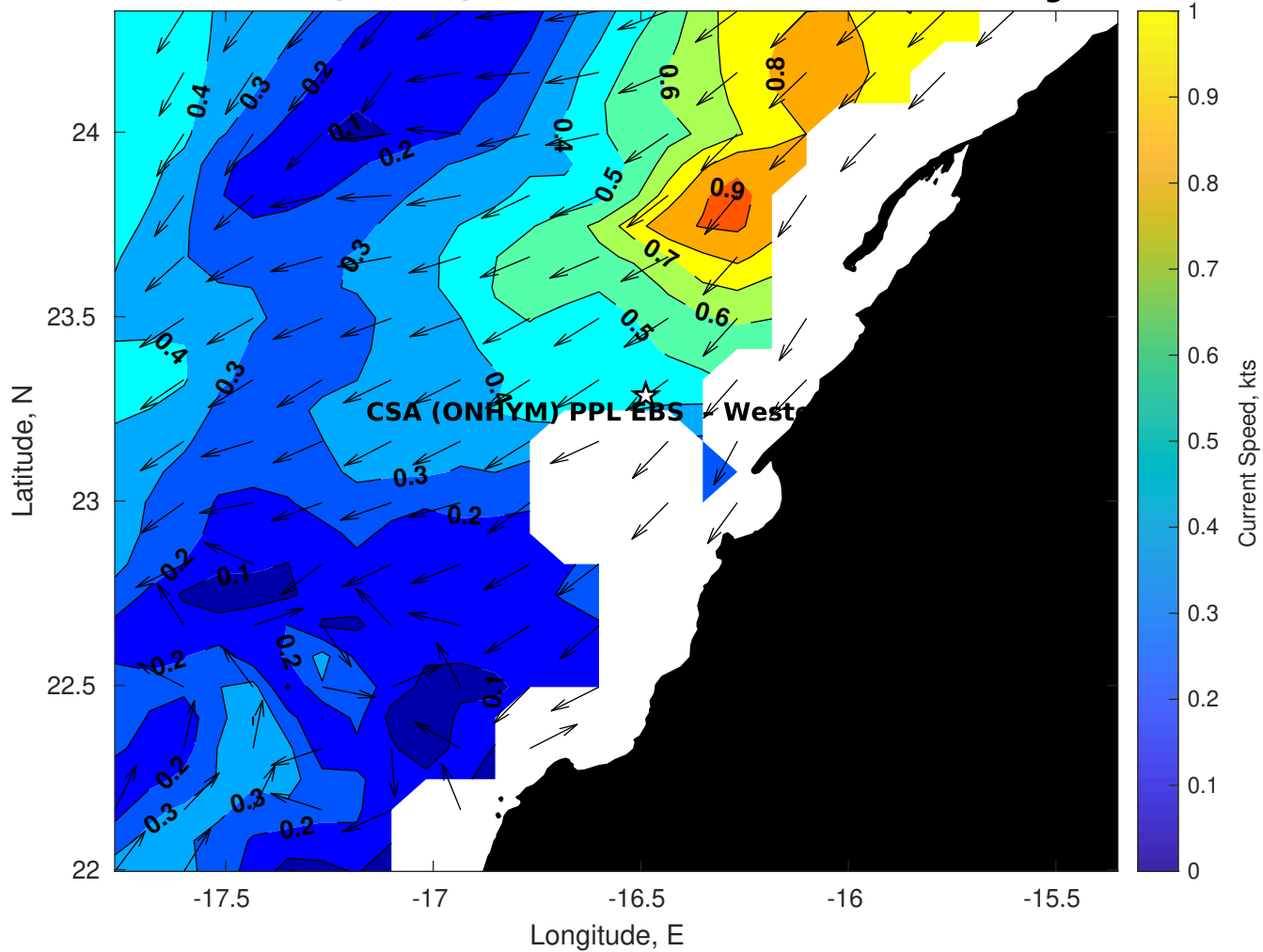
Surface Currents for CSA (ONHYM) PPL EBS - Western Sahara at 29-Aug-2025 00:00:00
