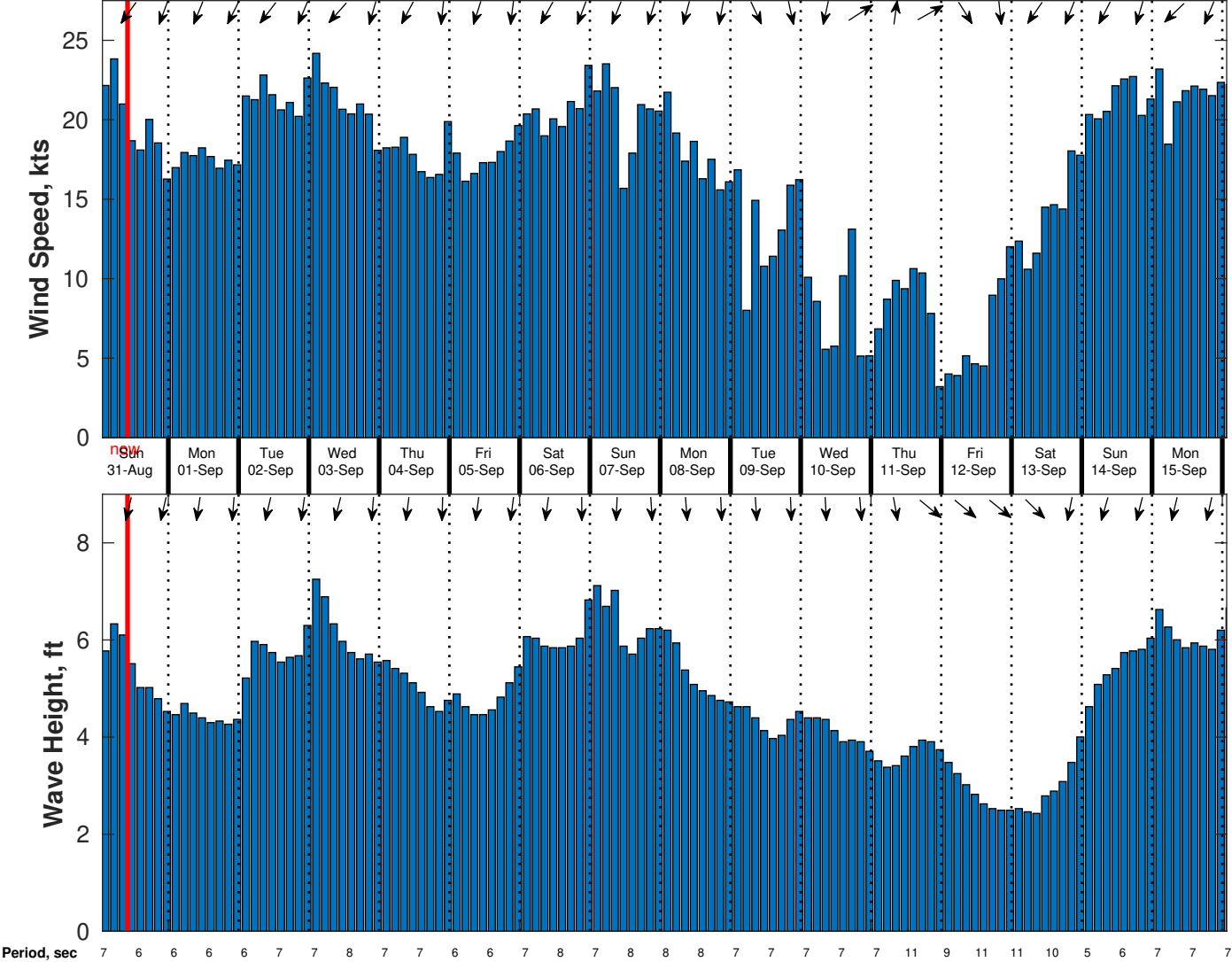
Wind & Wave Forecast for CSA (ONHYM) PPL EBS - Western Sahara from 30-Aug-2025 01:00:00 to 15-Sep-2025 01:00:00
