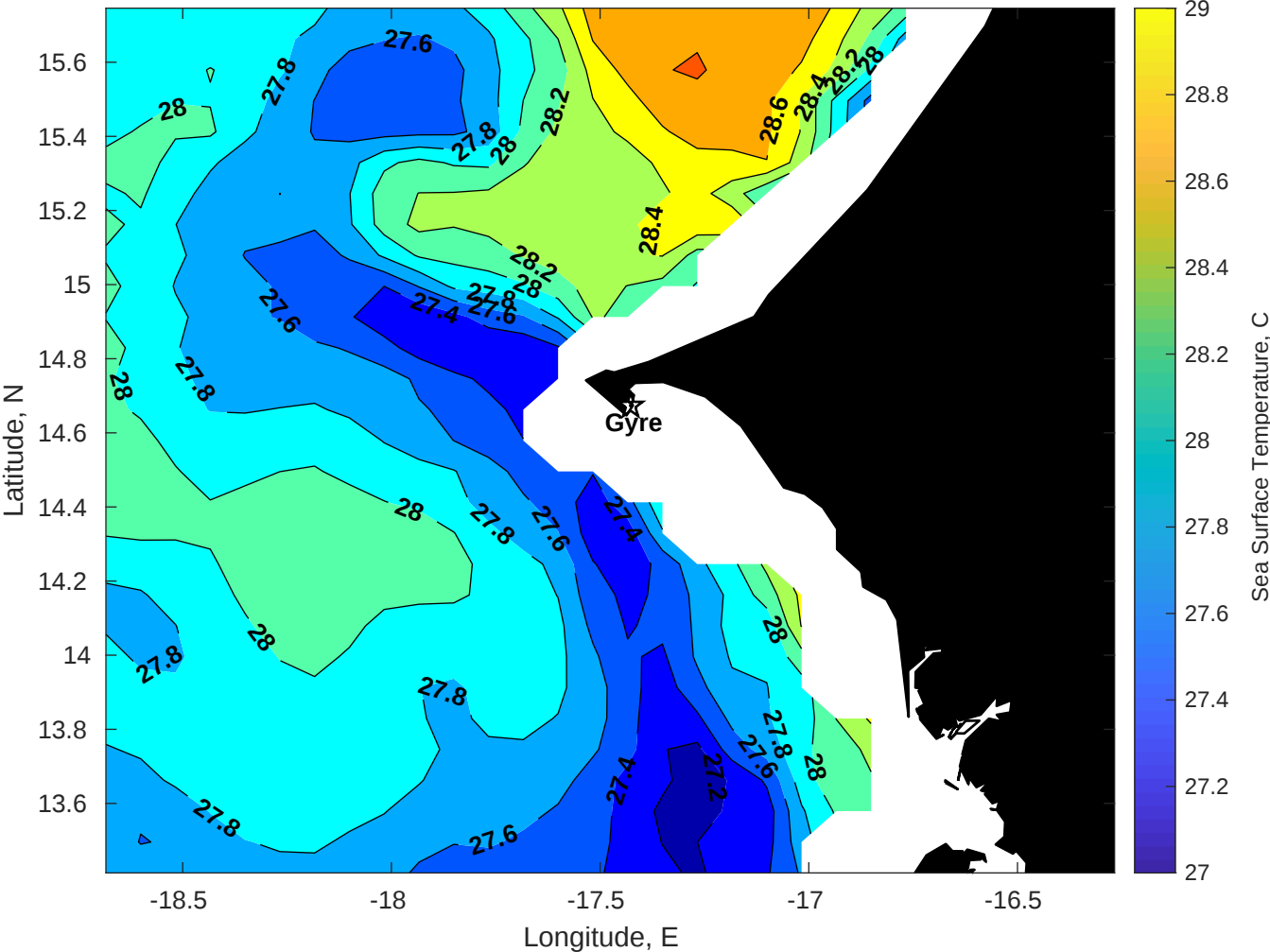
SST for Gyre at 29-Aug-2025 00:00:00
