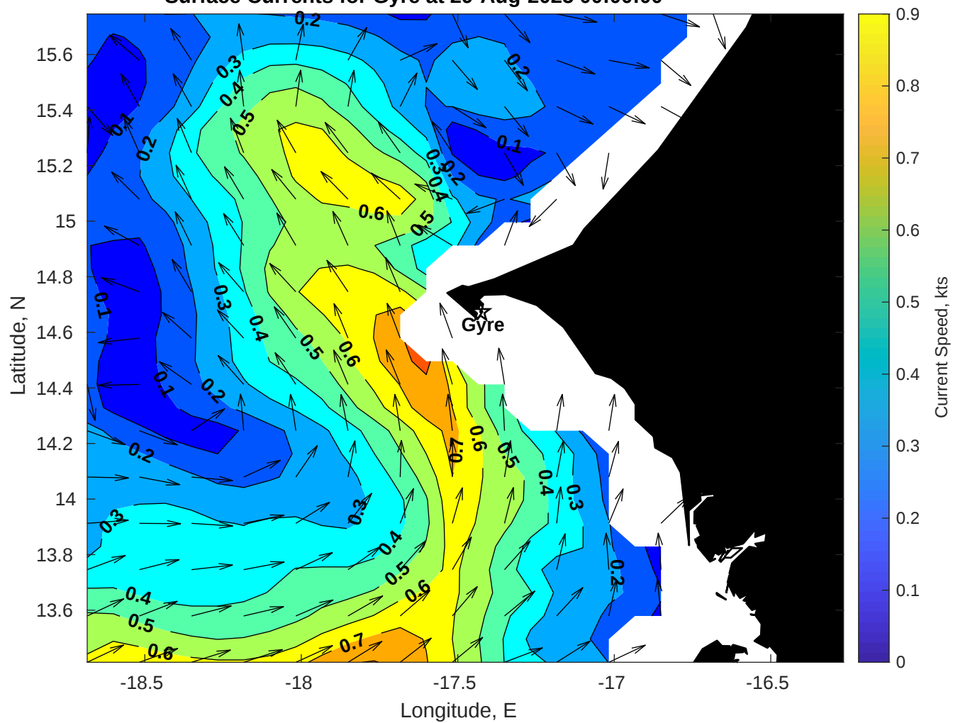
Surface Currents for Gyre at 29-Aug-2025 00:00:00
