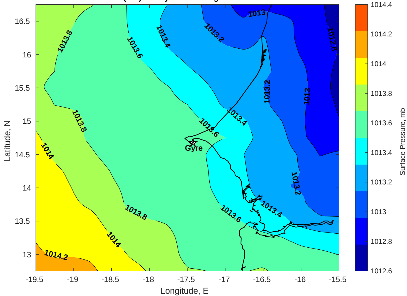
Surface Pressure (mb) for Gyre at 30-Aug-2025 00:00:00
