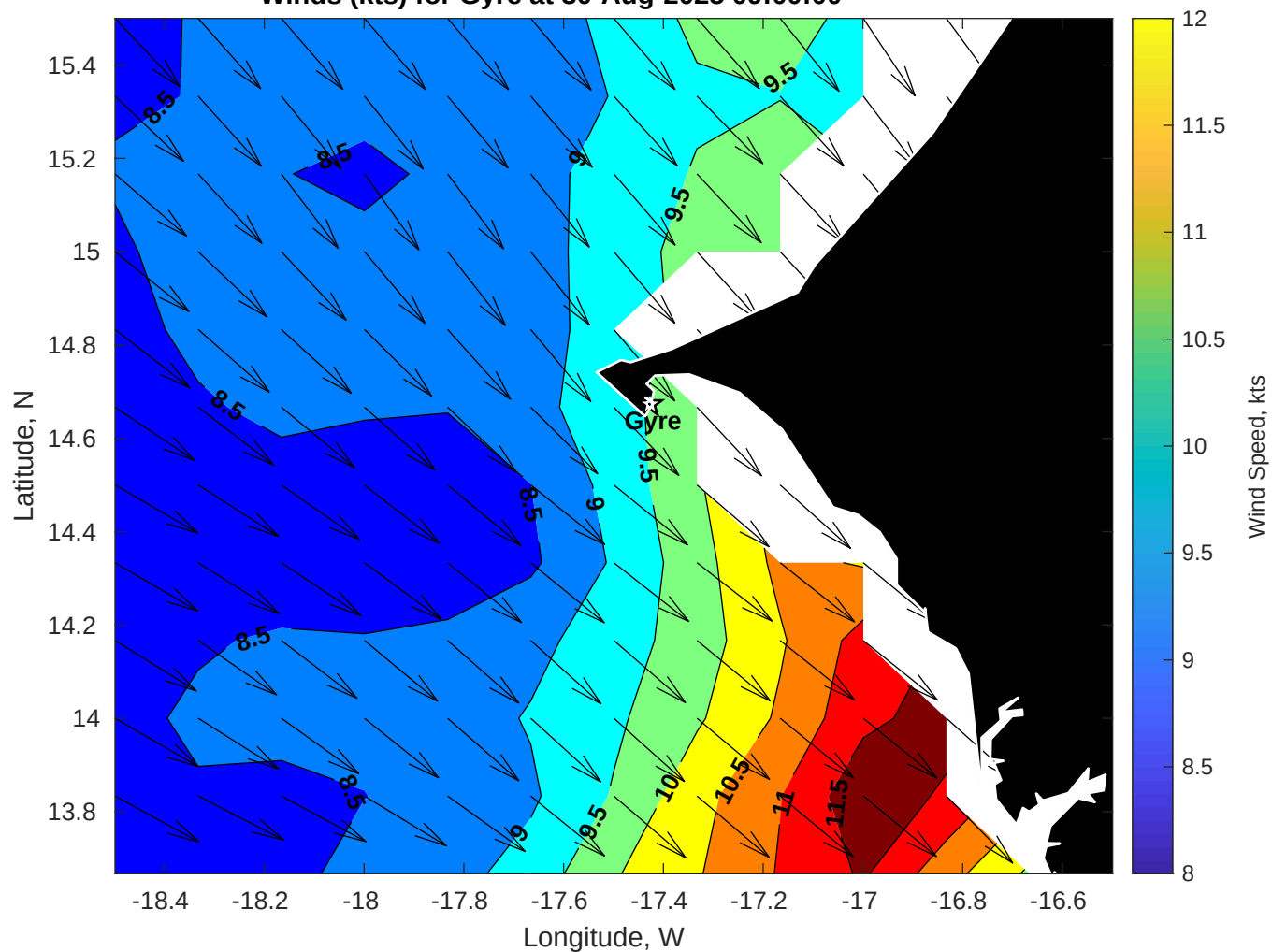
Winds (kts) for Gyre at 30-Aug-2025 09:00:00
