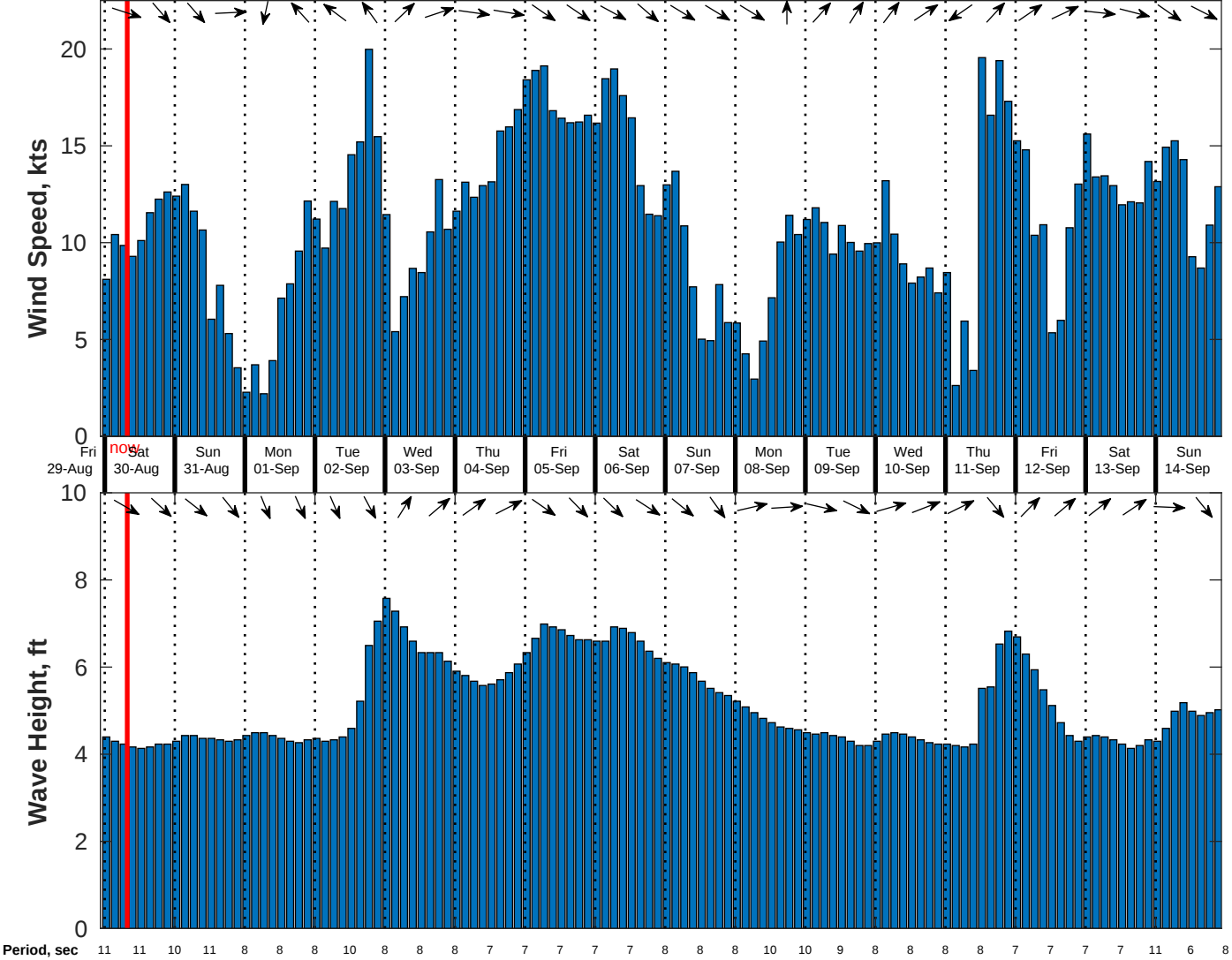
Wind & Wave Forecast for Gyre from 29-Aug-2025 23:00:00 to 14-Sep-2025 23:00:00
