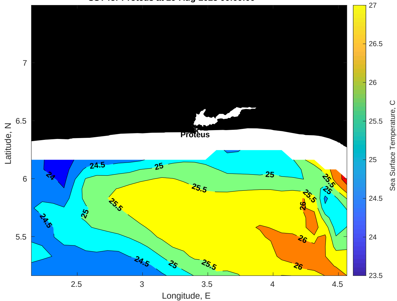
SST for Proteus at 29-Aug-2025 00:00:00
