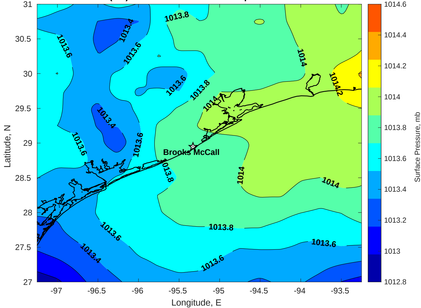
Surface Pressure (mb) for Brooks McCall at 02-Sep-2025 00:00:00
