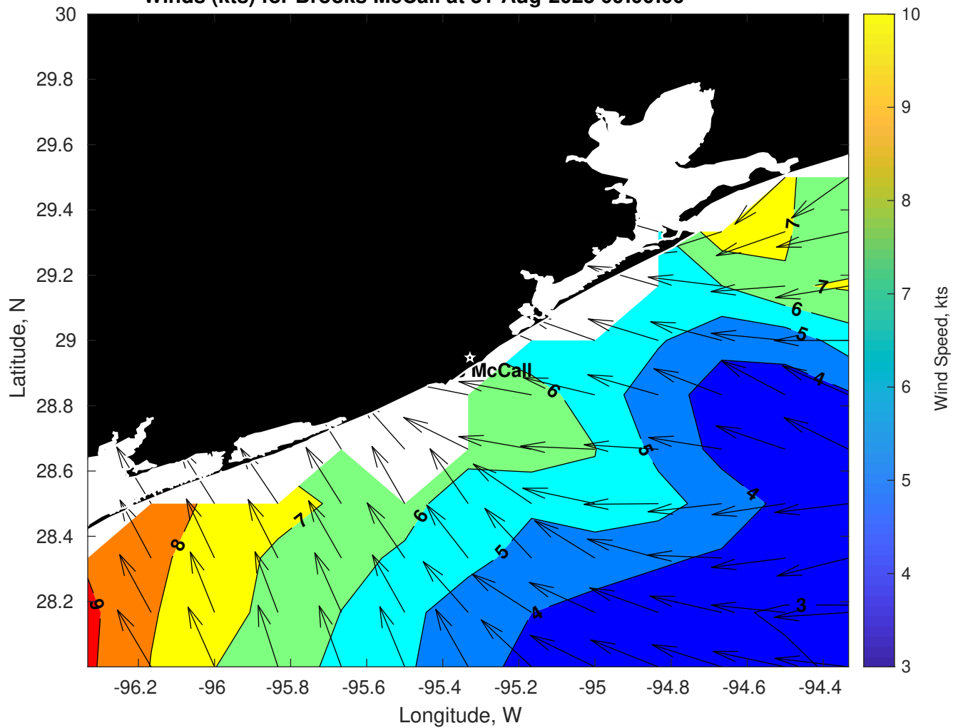
Winds (kts) for Brooks McCall at 31-Aug-2025 09:00:00
