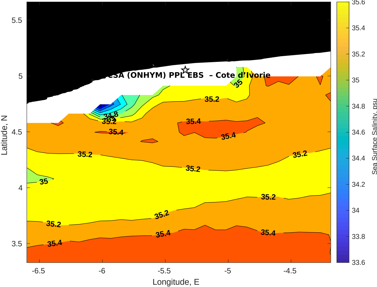
Surface Salinity for CSA (ONHYM) PPL EBS - Cote d'Ivoire at 30-Aug-2025 00:00:00
