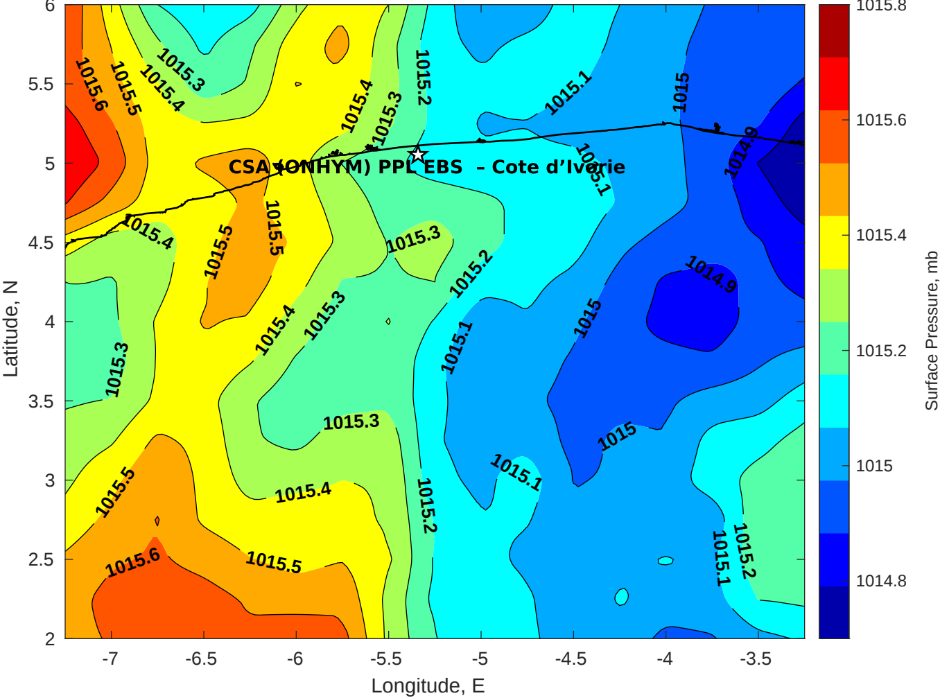
Surface Pressure (mb) for CSA (ONHYM) PPL EBS - Cote d'Ivoire at 02-Sep-2025 00:00:00
