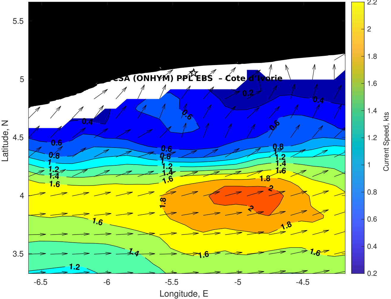
Surface Currents for CSA (ONHYM) PPL EBS - Cote d'Ivoire at 30-Aug-2025 00:00:00
