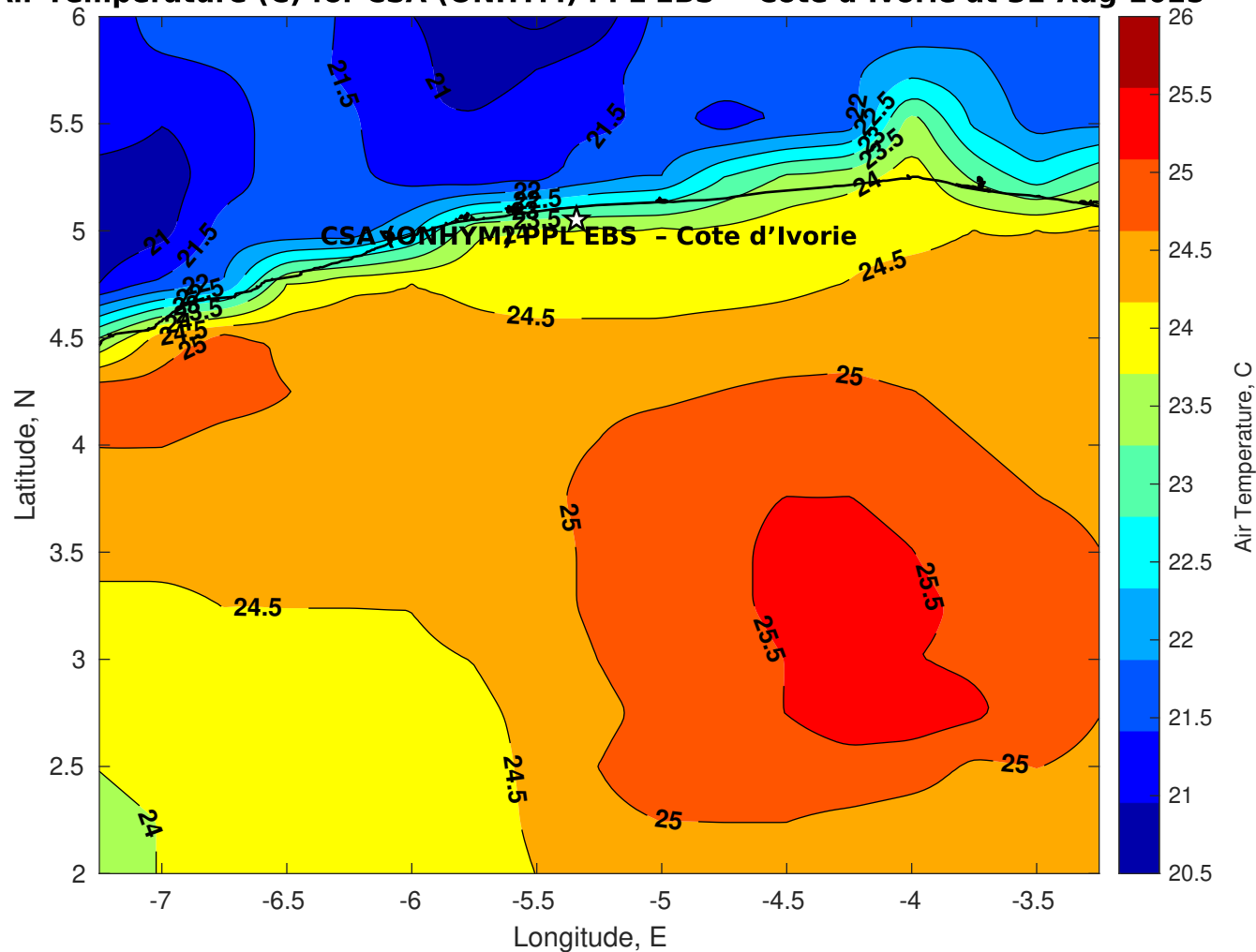
Air Temperature (C) for CSA (ONHYM) PPL EBS - Cote d'Ivoire at 31-Aug-2025
