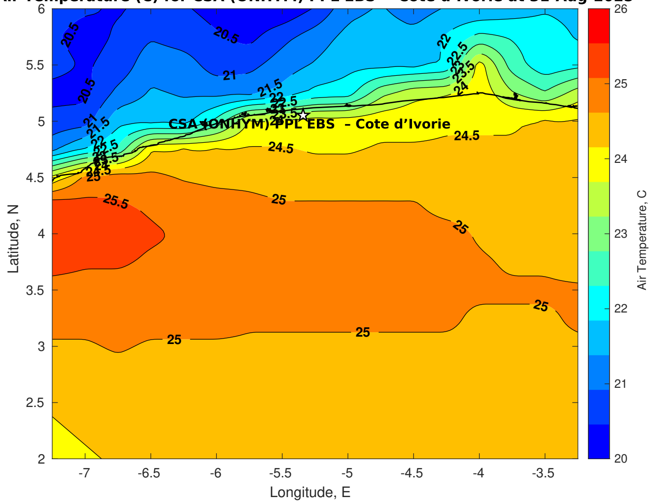
Air Temperature (C) for CSA (ONHYM) PPL EBS - Cote d'Ivoire at 31-Aug-2025
