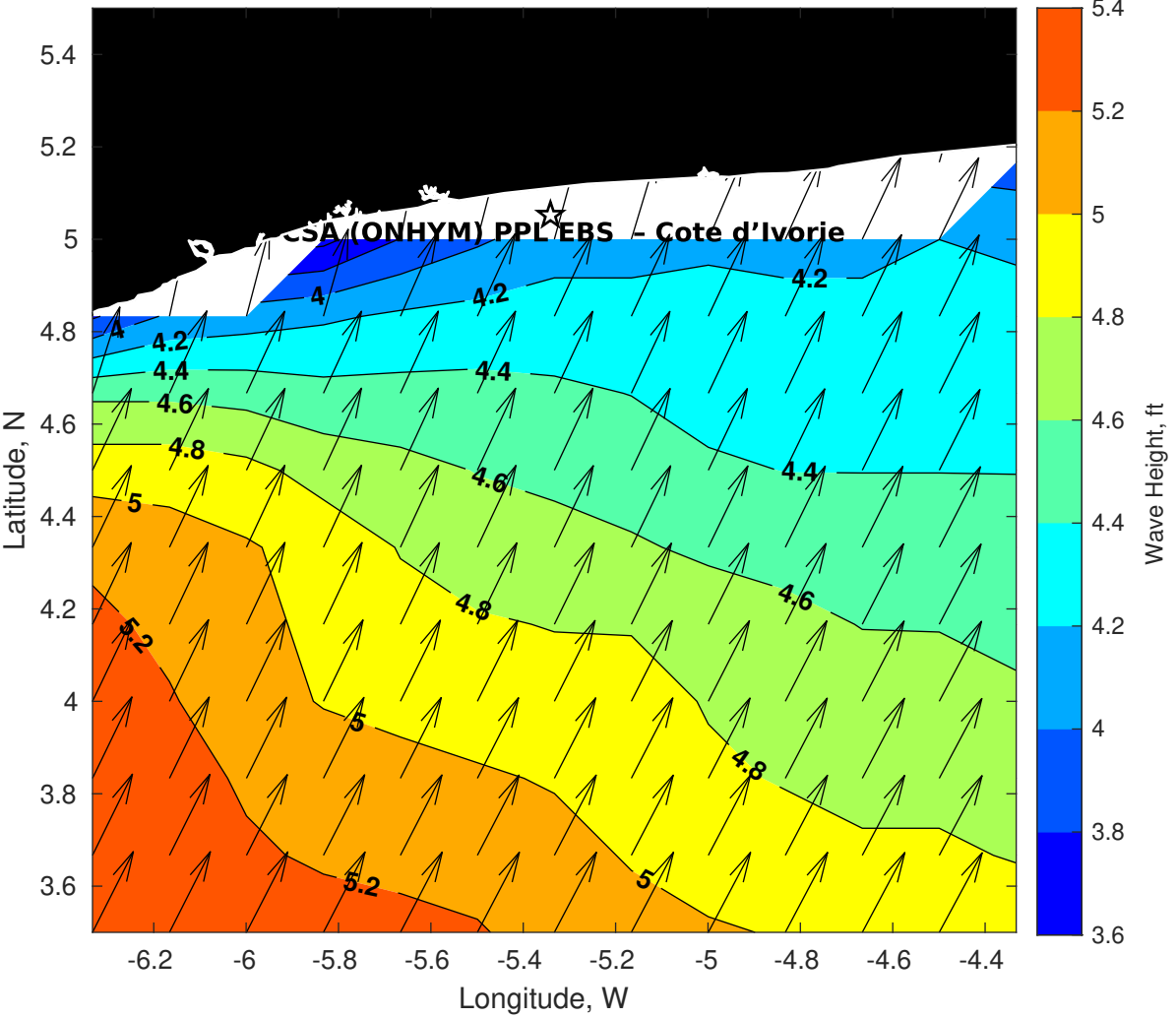
Wave Height (ft) for CSA (ONHYM) PPL EBS - Cote d'Ivoire at 31-Aug-2025 09:00:00
