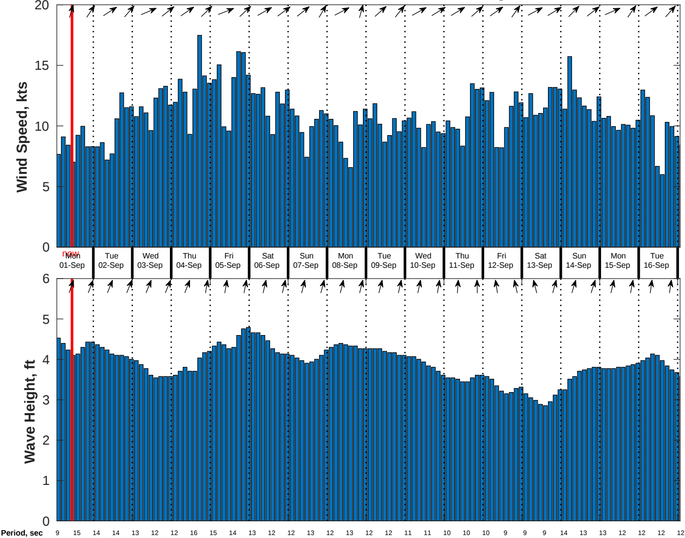
Wind & Wave Forecast for CSA (ONHYM) PPL EBS - Cote d'Ivoire from 31-Aug-2025 01:00:00 to 16-Sep-2025 01:00:00
