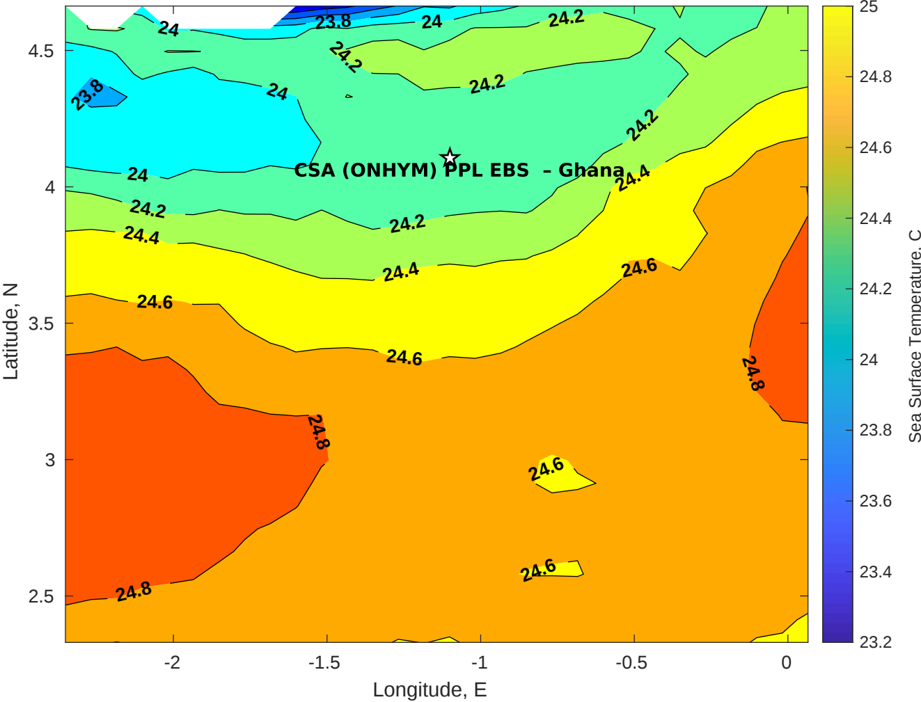
SST for CSA (ONHYM) PPL EBS - Ghana at 30-Aug-2025 00:00:00
