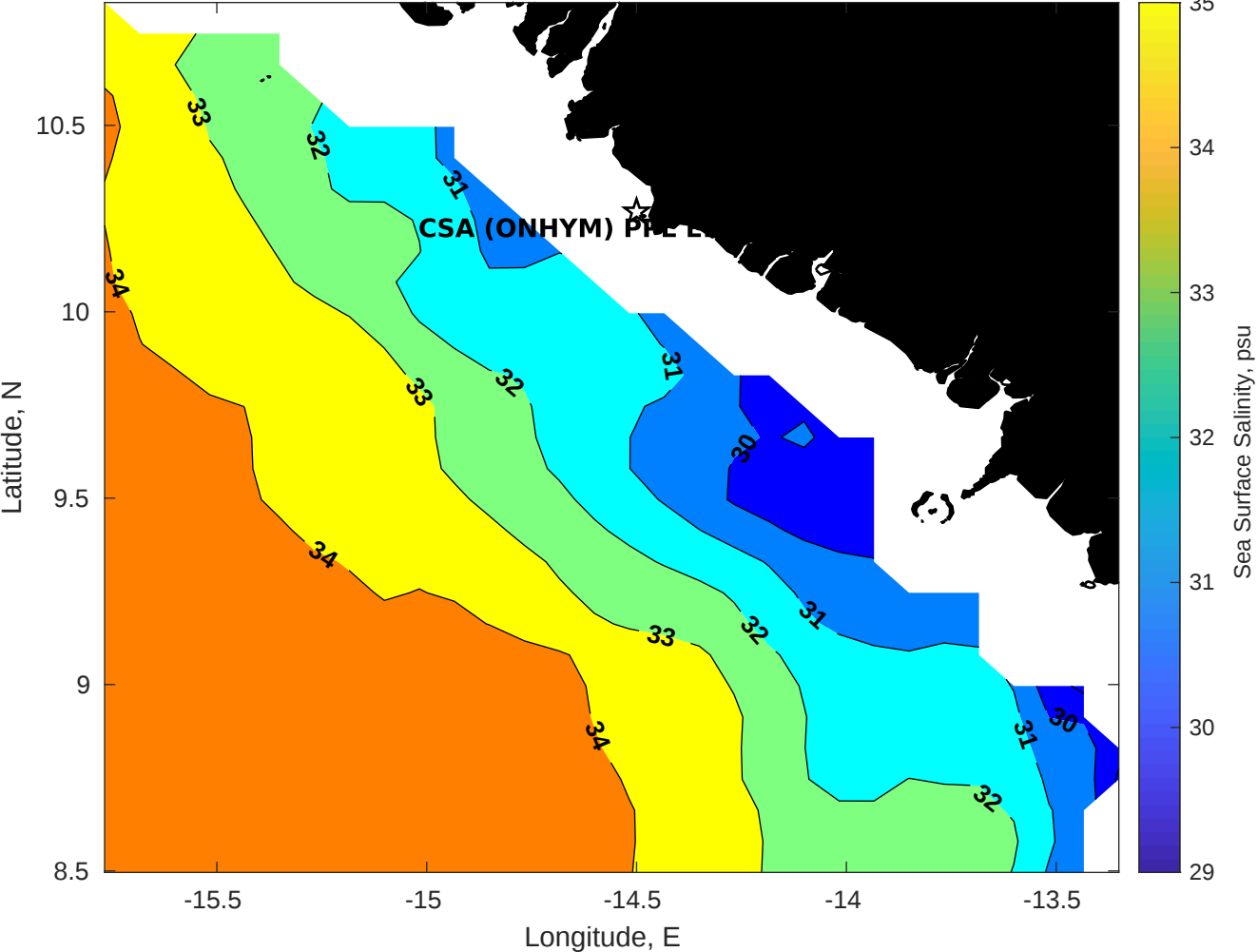
Surface Salinity for CSA (ONHYM) PPL EBS - Guinea at 30-Aug-2025 00:00:00
