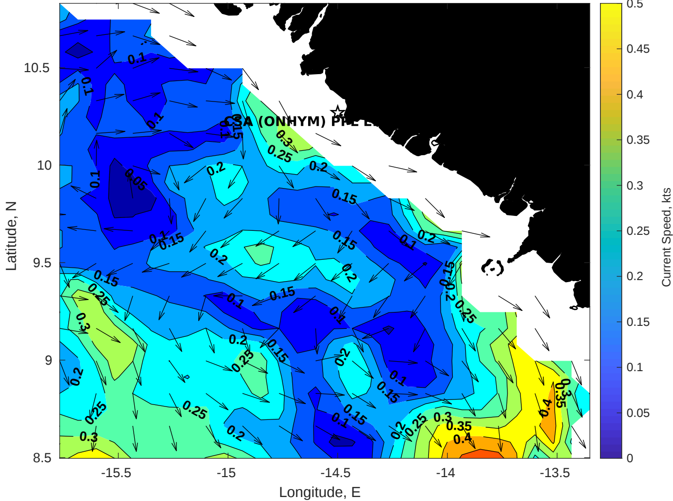
Surface Currents for CSA (ONHYM) PPL EBS - Guinea at 30-Aug-2025 00:00:00
