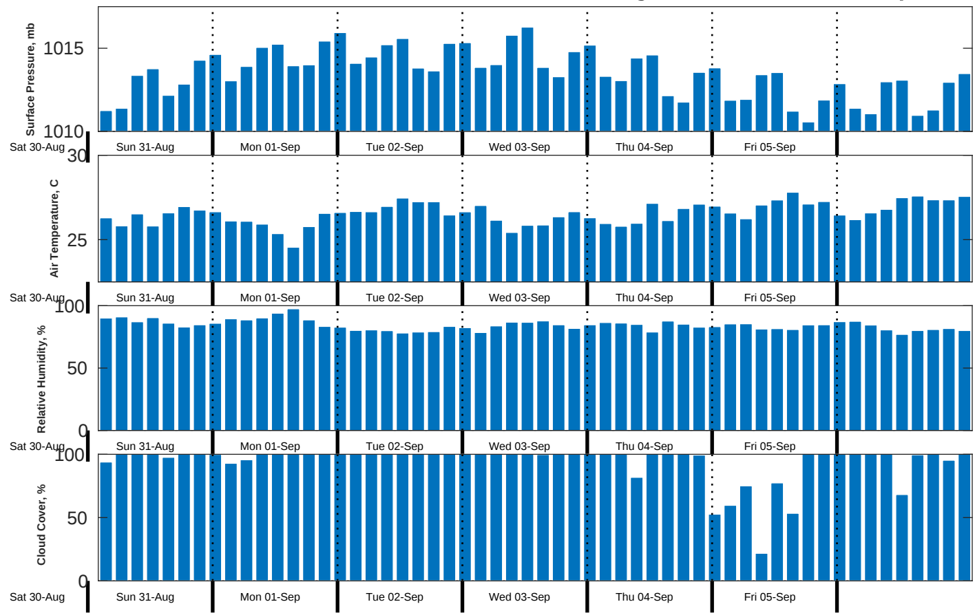
Met Forecast for CSA (ONHYM) PPL EBS - Guinea from 31-Aug-2025 00:00:00 to 07-Sep-2025 00:00:00
