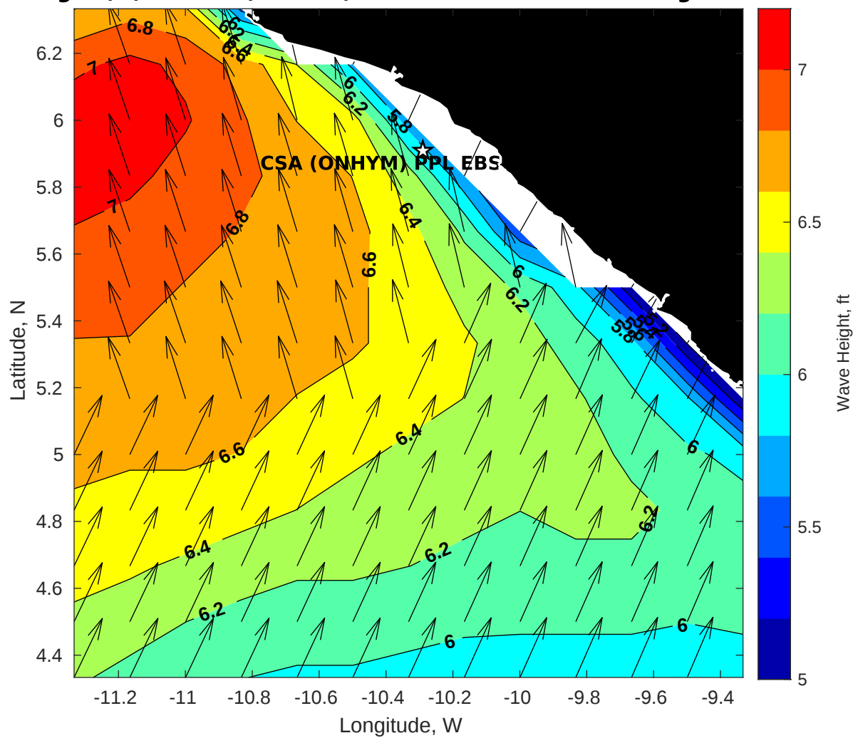
Wave Height (ft) for CSA (ONHYM) PPL EBS - Liberia at 31-Aug-2025 09:00:00
