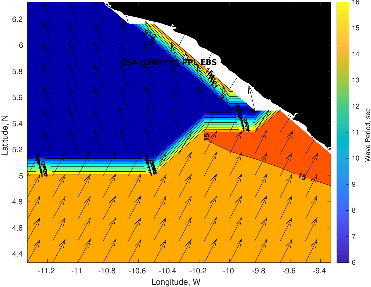
Wave Period (sec) for CSA (ONHYM) PPL EBS - Liberia at 31-Aug-2025 09:00:00
