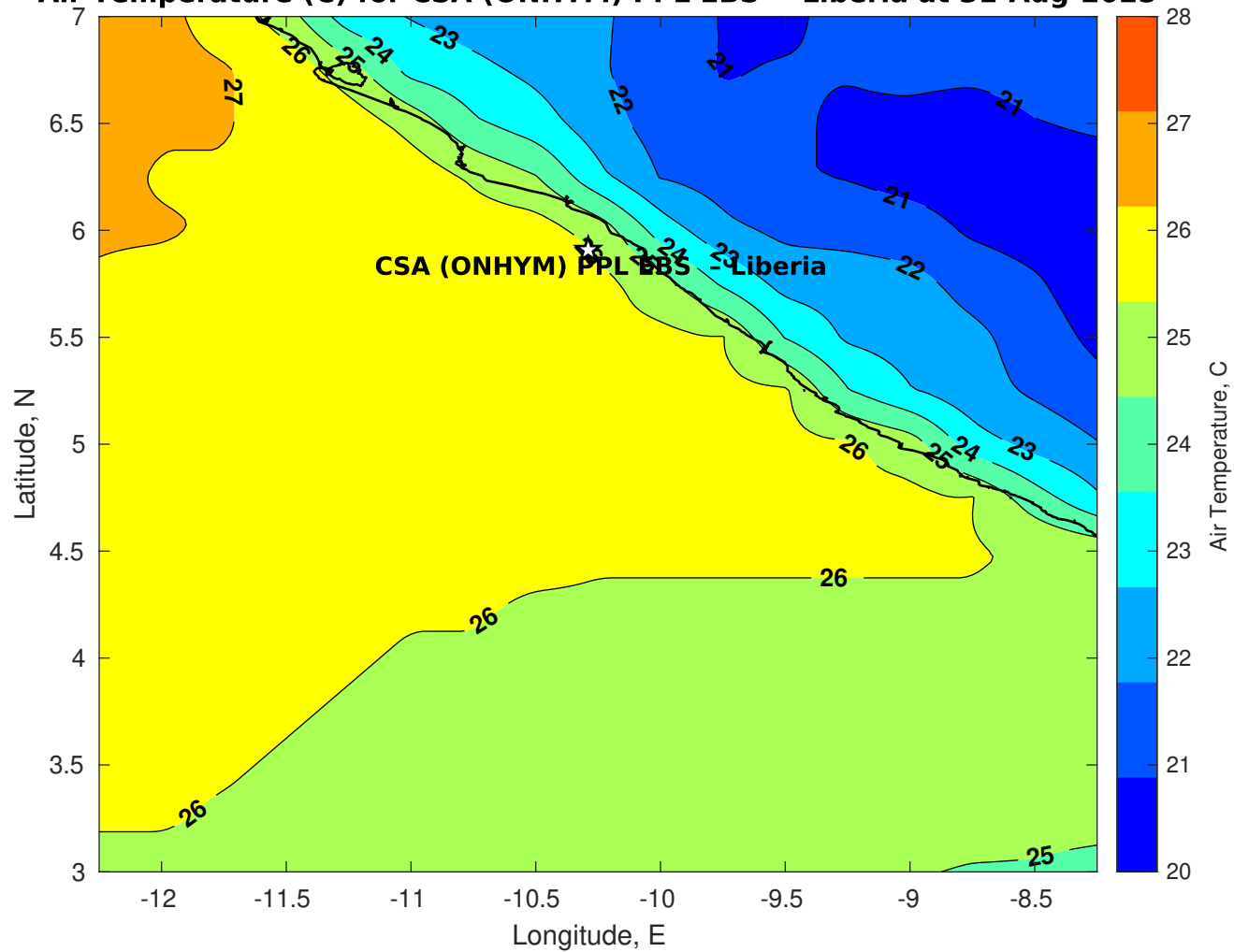
Air Temperature (C) for CSA (ONHYM) PPL EBS - Liberia at 31-Aug-2025
