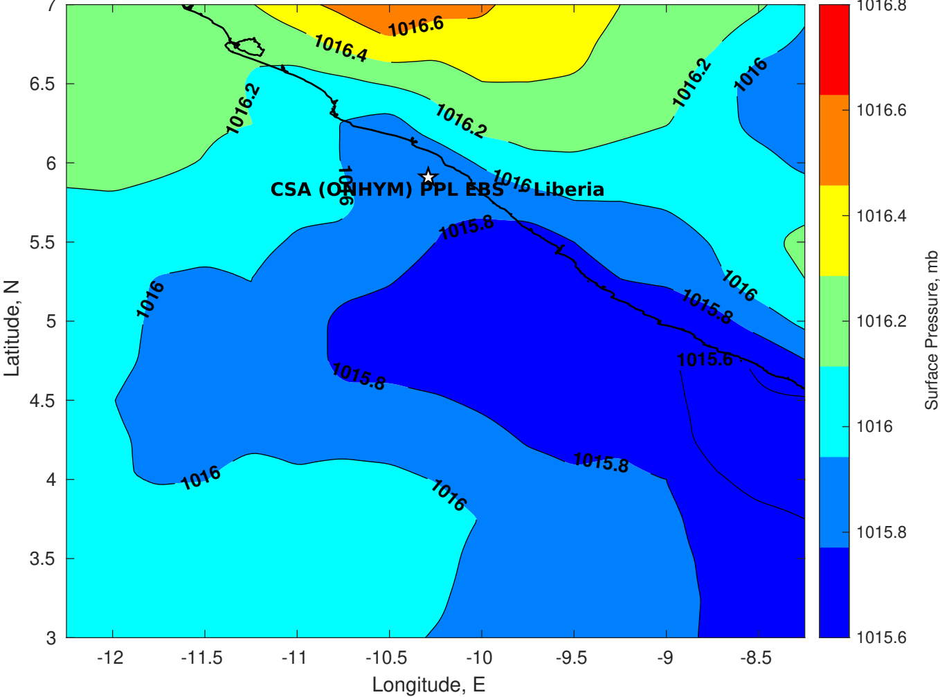
Surface Pressure (mb) for CSA (ONHYM) PPL EBS - Liberia at 02-Sep-2025 00:00:00
