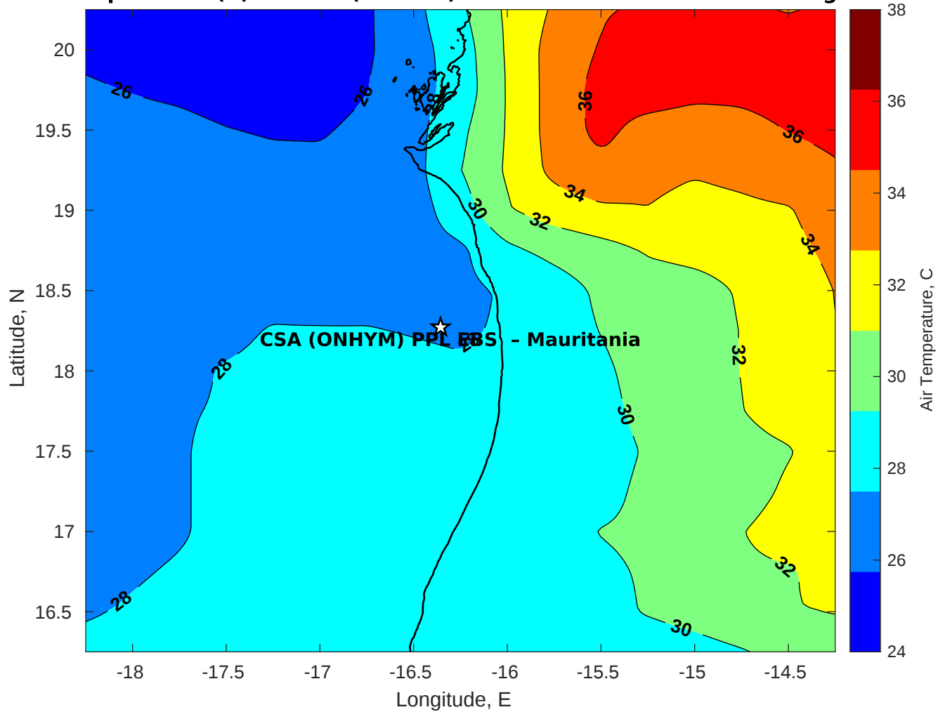
Air Temperature (C) for CSA (ONHYM) PPL EBS - Mauritania at 31-Aug-2025
