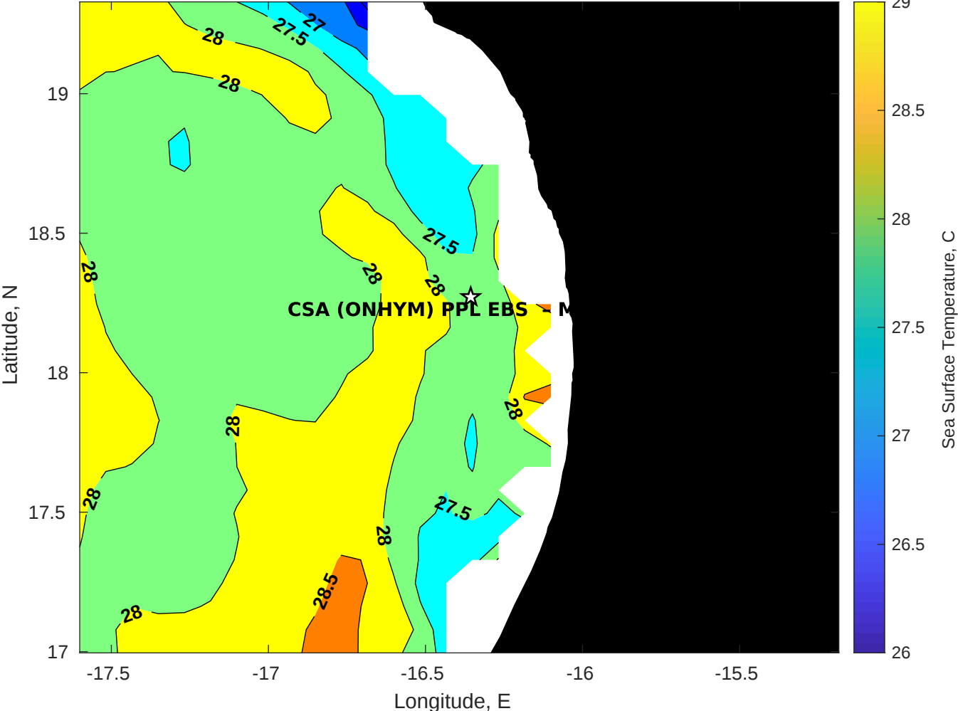
SST for CSA (ONHYM) PPL EBS - Mauritania at 30-Aug-2025 00:00:00
