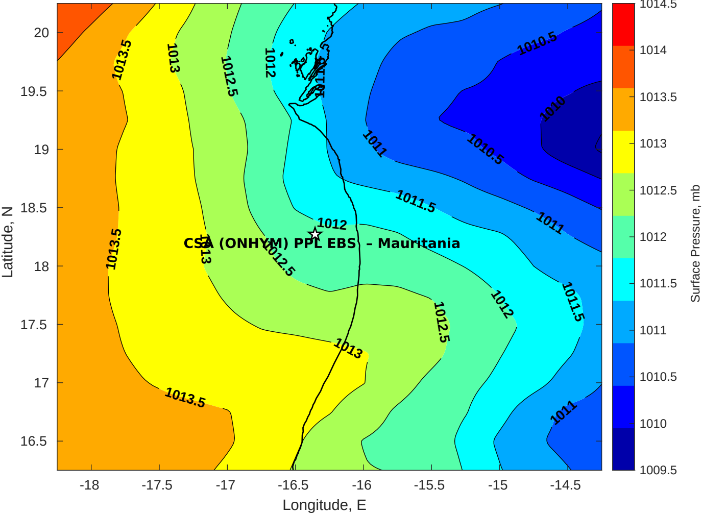
Surface Pressure (mb) for CSA (ONHYM) PPL EBS - Mauritania at 31-Aug-2025 00:00:00
