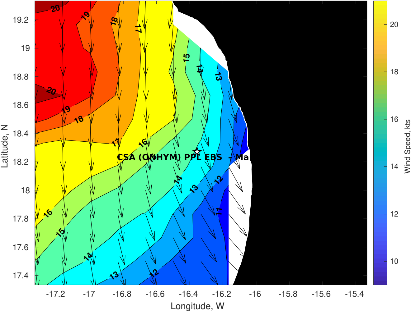
Winds (kts) for CSA (ONHYM) PPL EBS - Mauritania at 31-Aug-2025 09:00:00
