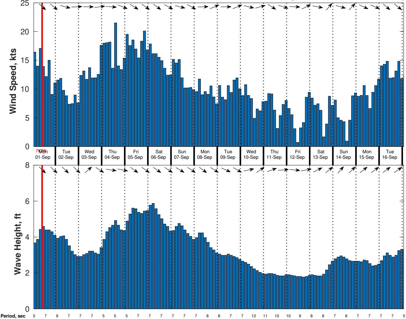
Wind & Wave Forecast for CSA (ONHYM) PPL EBS - Mauritania from 31-Aug-2025 01:00:00 to 16-Sep-2025 01:00:00
