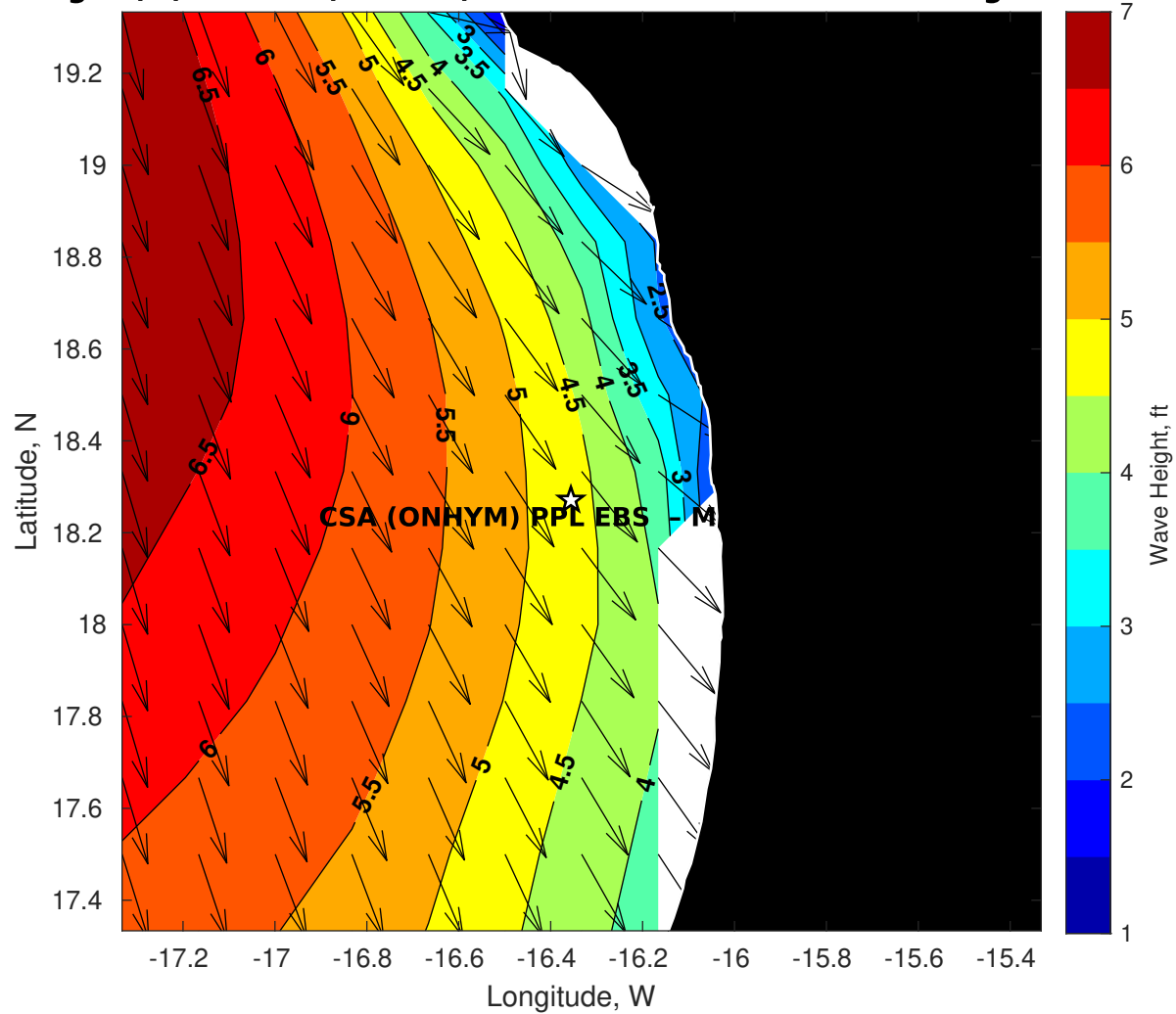
Wave Height (ft) for CSA (ONHYM) PPL EBS - Mauritania at 31-Aug-2025 09:00:00
