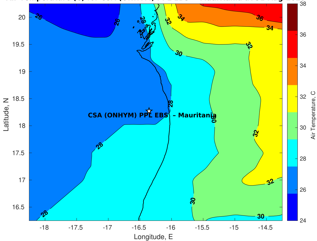
Air Temperature (C) for CSA (ONHYM) PPL EBS - Mauritania at 31-Aug-2025
