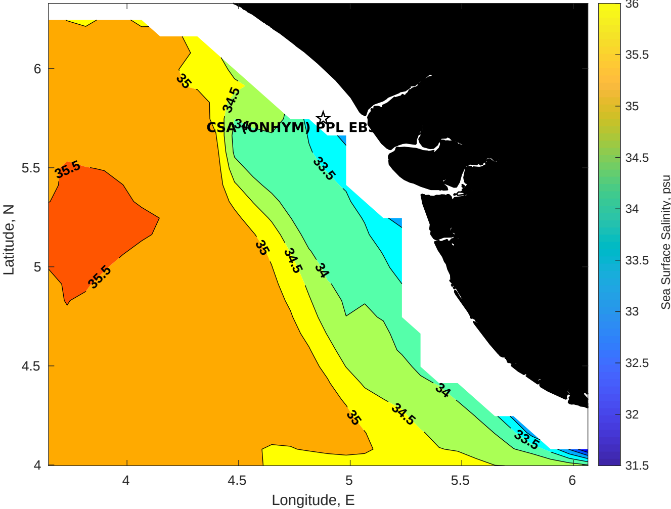
Surface Salinity for CSA (ONHYM) PPL EBS - Nigeria at 30-Aug-2025 00:00:00
