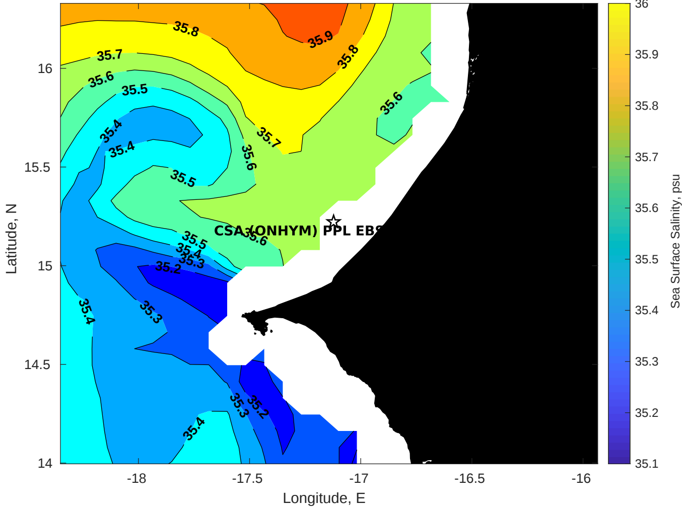
Surface Salinity for CSA (ONHYM) PPL EBS - Senegal at 30-Aug-2025 00:00:00
