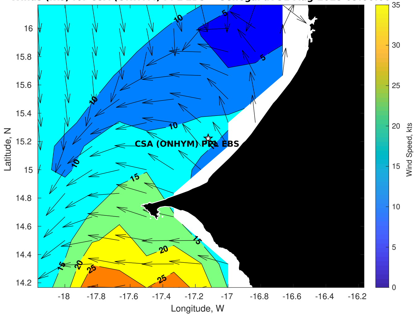
Winds (kts) for CSA (ONHYM) PPL EBS - Senegal at 31-Aug-2025 09:00:00
