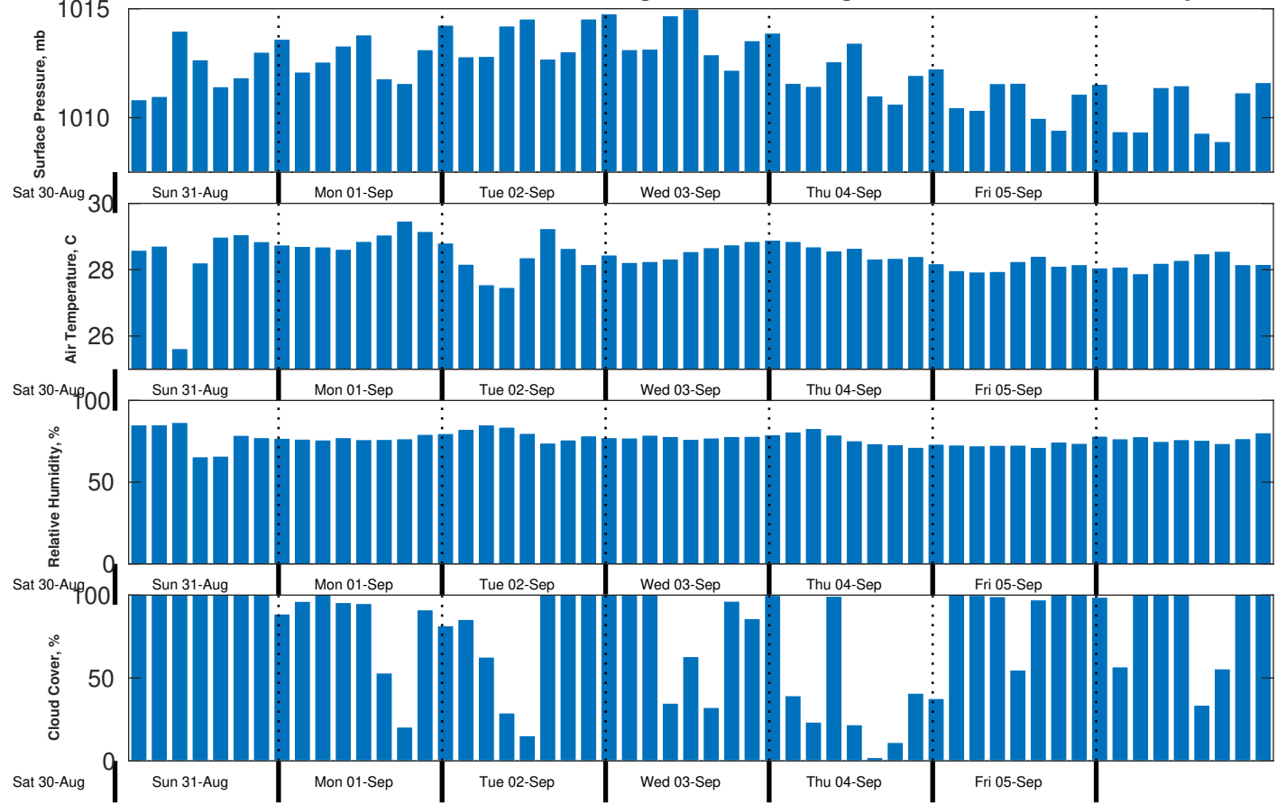
Met Forecast for CSA (ONHYM) PPL EBS - Senegal from 31-Aug-2025 00:00:00 to 07-Sep-2025 00:00:00
