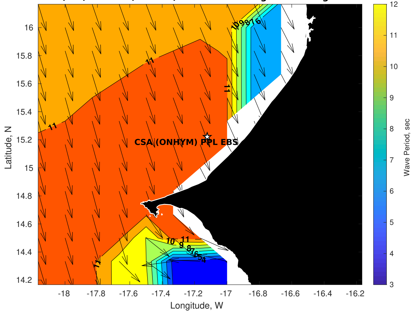
Wave Period (sec) for CSA (ONHYM) PPL EBS - Senegal at 31-Aug-2025 09:00:00
