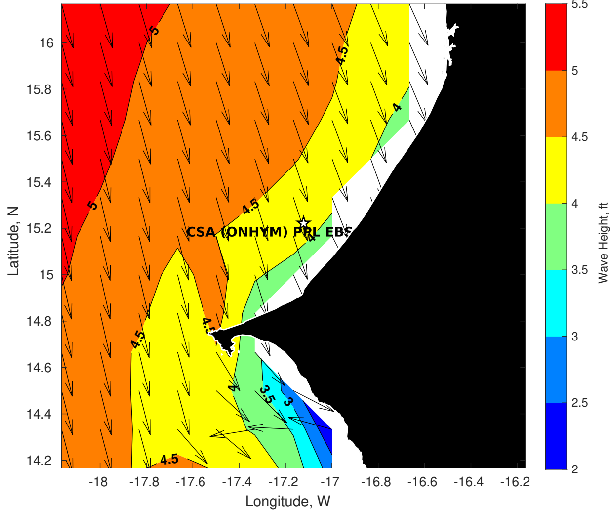
Wave Height (ft) for CSA (ONHYM) PPL EBS - Senegal at 31-Aug-2025 09:00:00
