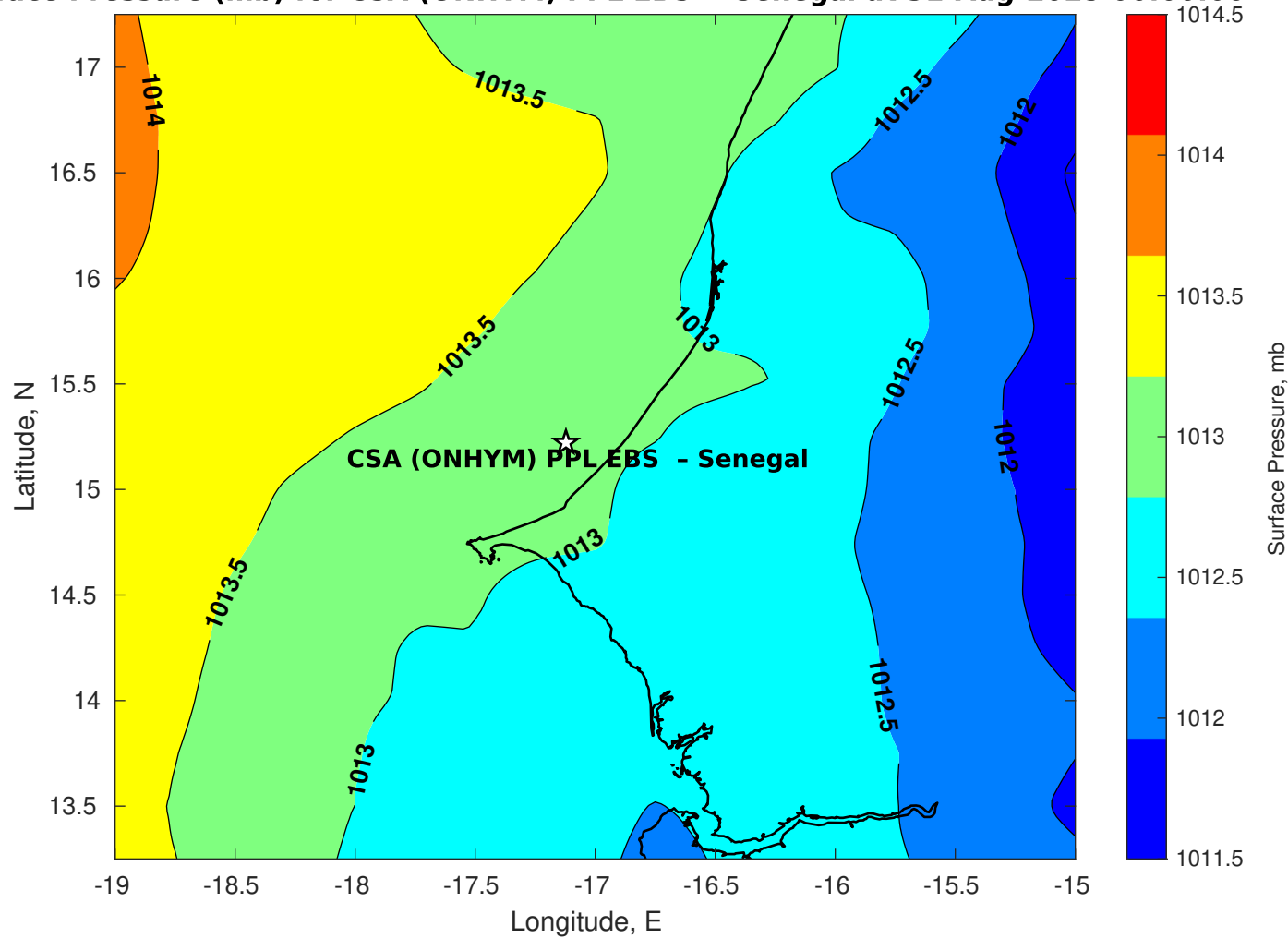
Surface Pressure (mb) for CSA (ONHYM) PPL EBS - Senegal at 31-Aug-2025 00:00:00
