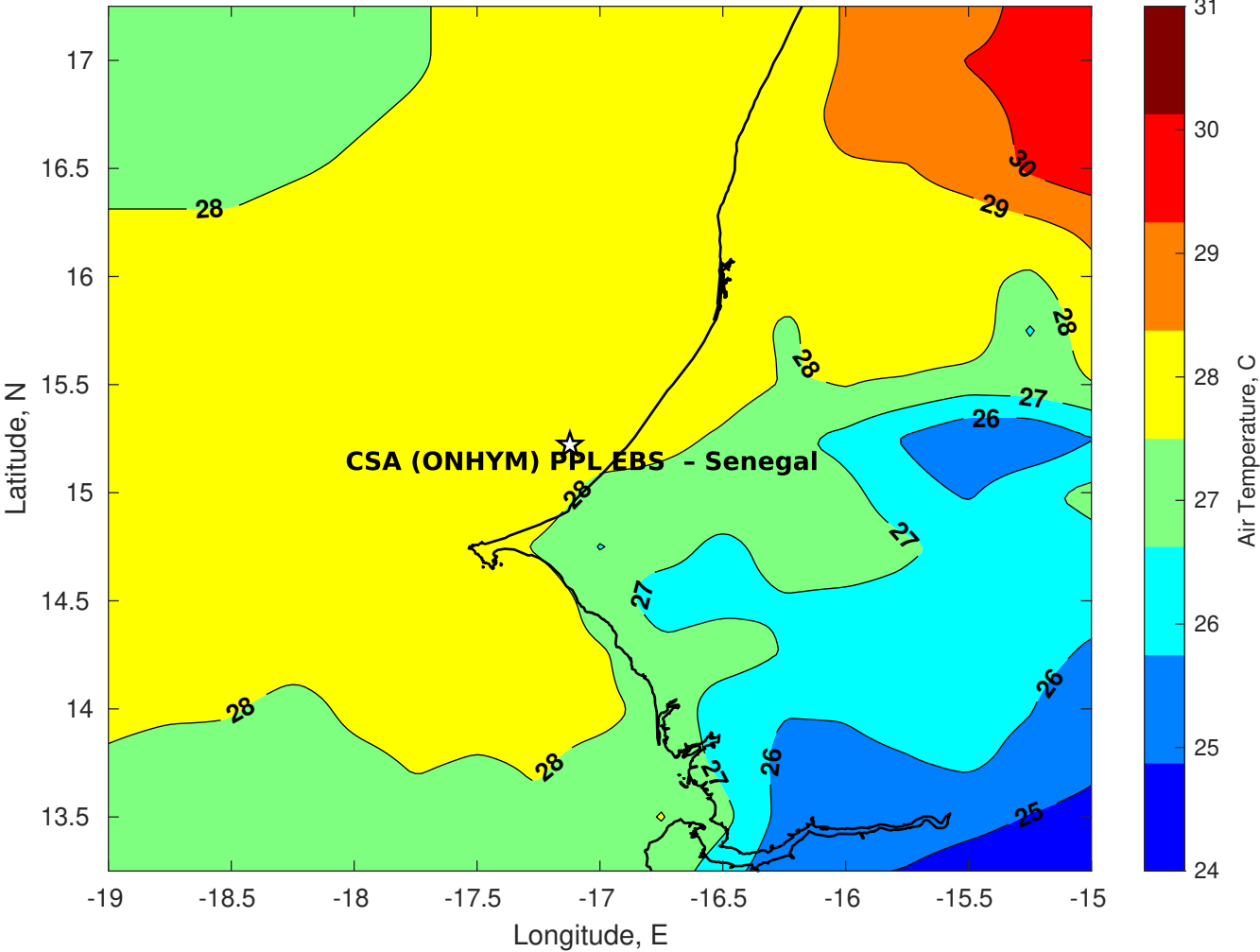
Air Temperature (C) for CSA (ONHYM) PPL EBS - Senegal at 31-Aug-2025
