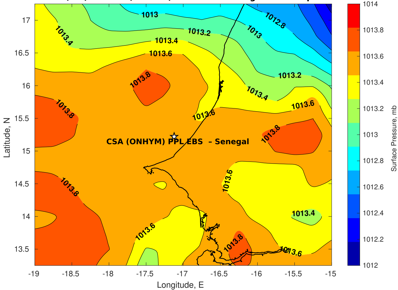
Surface Pressure (mb) for CSA (ONHYM) PPL EBS - Senegal at 01-Sep-2025 00:00:00
