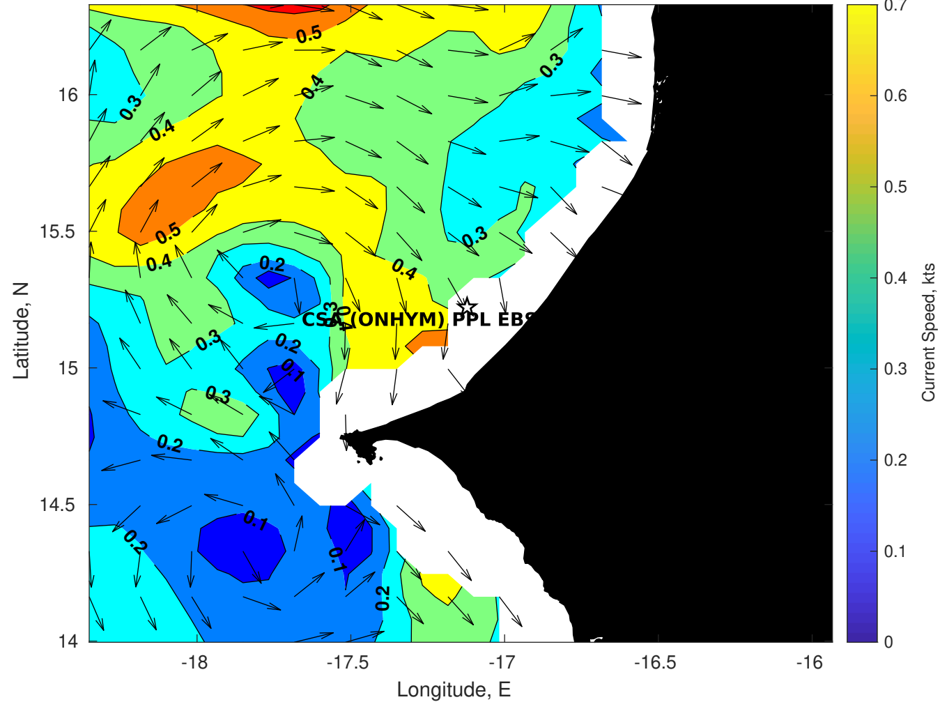
Surface Currents for CSA (ONHYM) PPL EBS - Senegal at 30-Aug-2025 00:00:00
