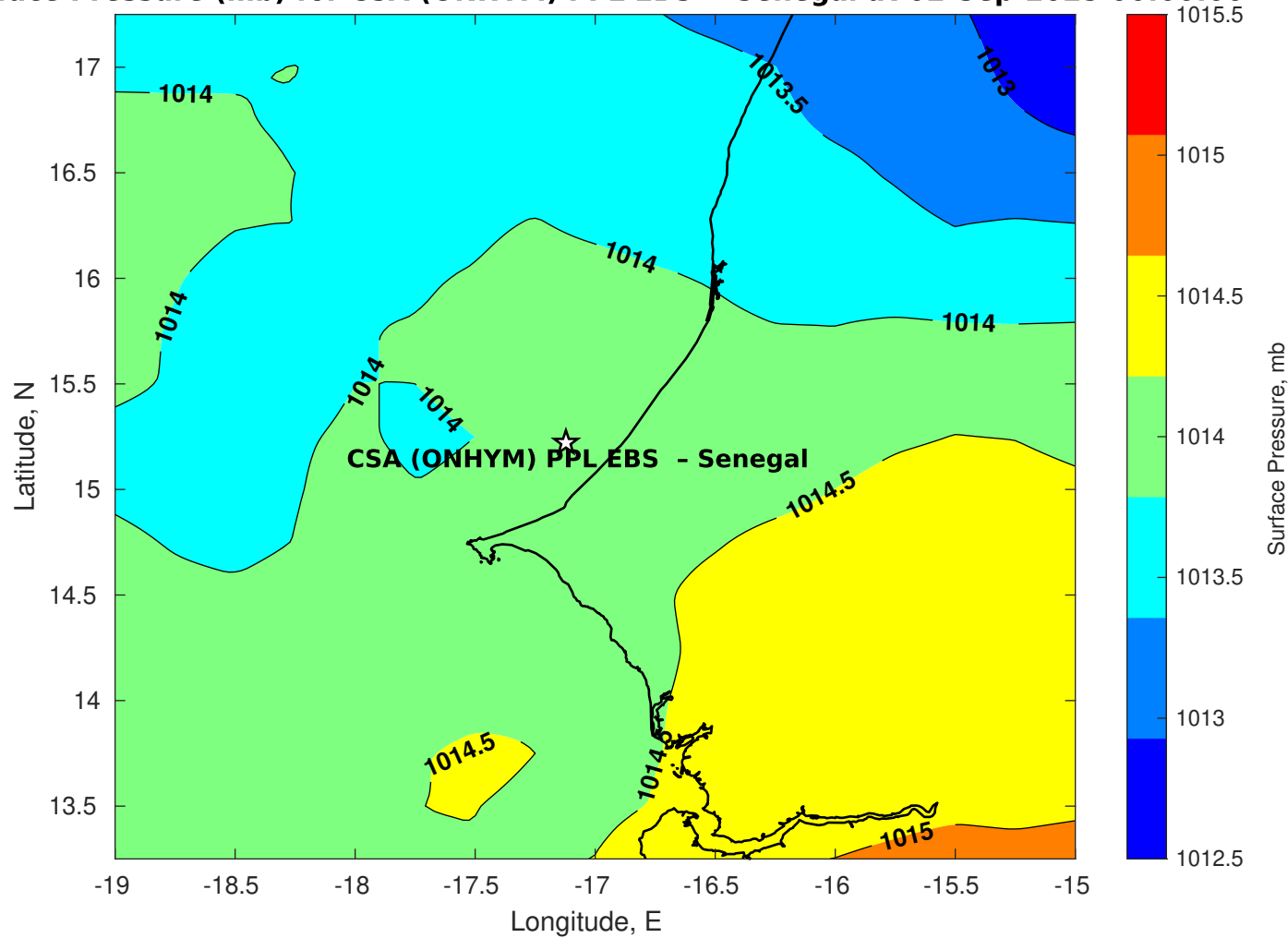
Surface Pressure (mb) for CSA (ONHYM) PPL EBS - Senegal at 02-Sep-2025 00:00:00
