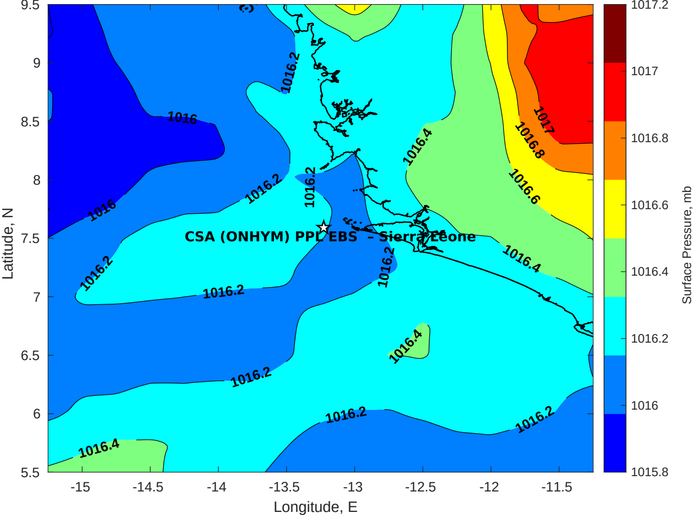
Surface Pressure (mb) for CSA (ONHYM) PPL EBS - Sierra Leone at 02-Sep-2025 00:00:00
