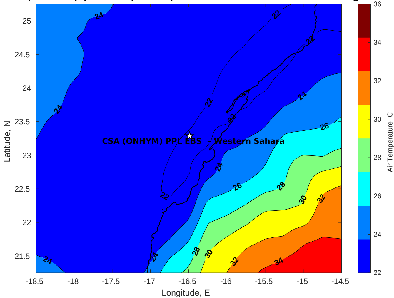
Air Temperature (C) for CSA (ONHYM) PPL EBS - Western Sahara at 31-Aug-2025
