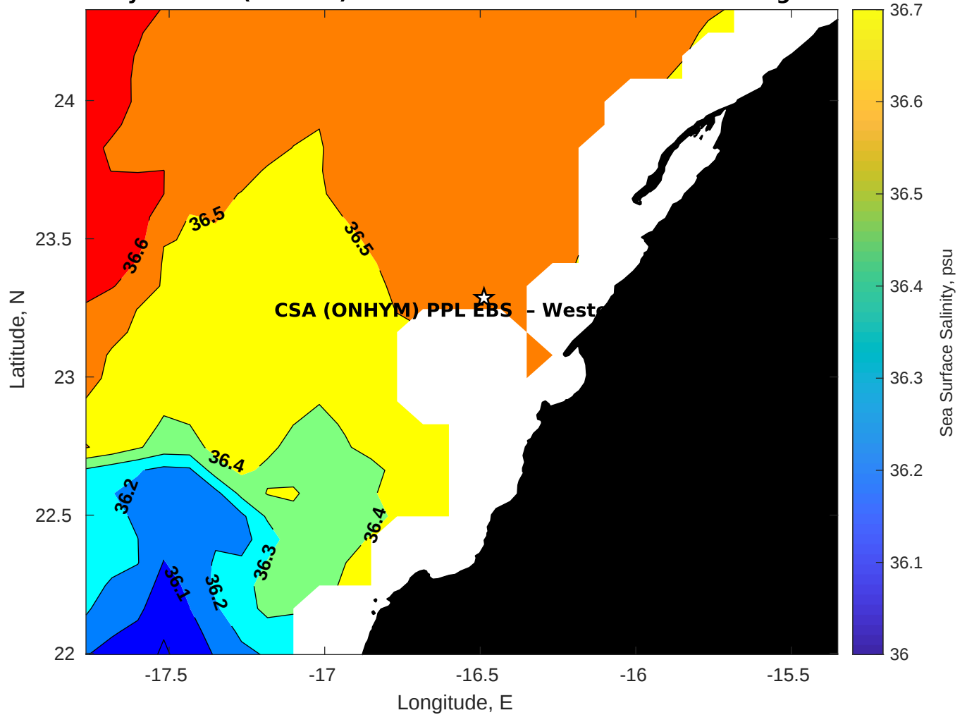
Surface Salinity for CSA (ONHYM) PPL EBS - Western Sahara at 30-Aug-2025 00:00:00
