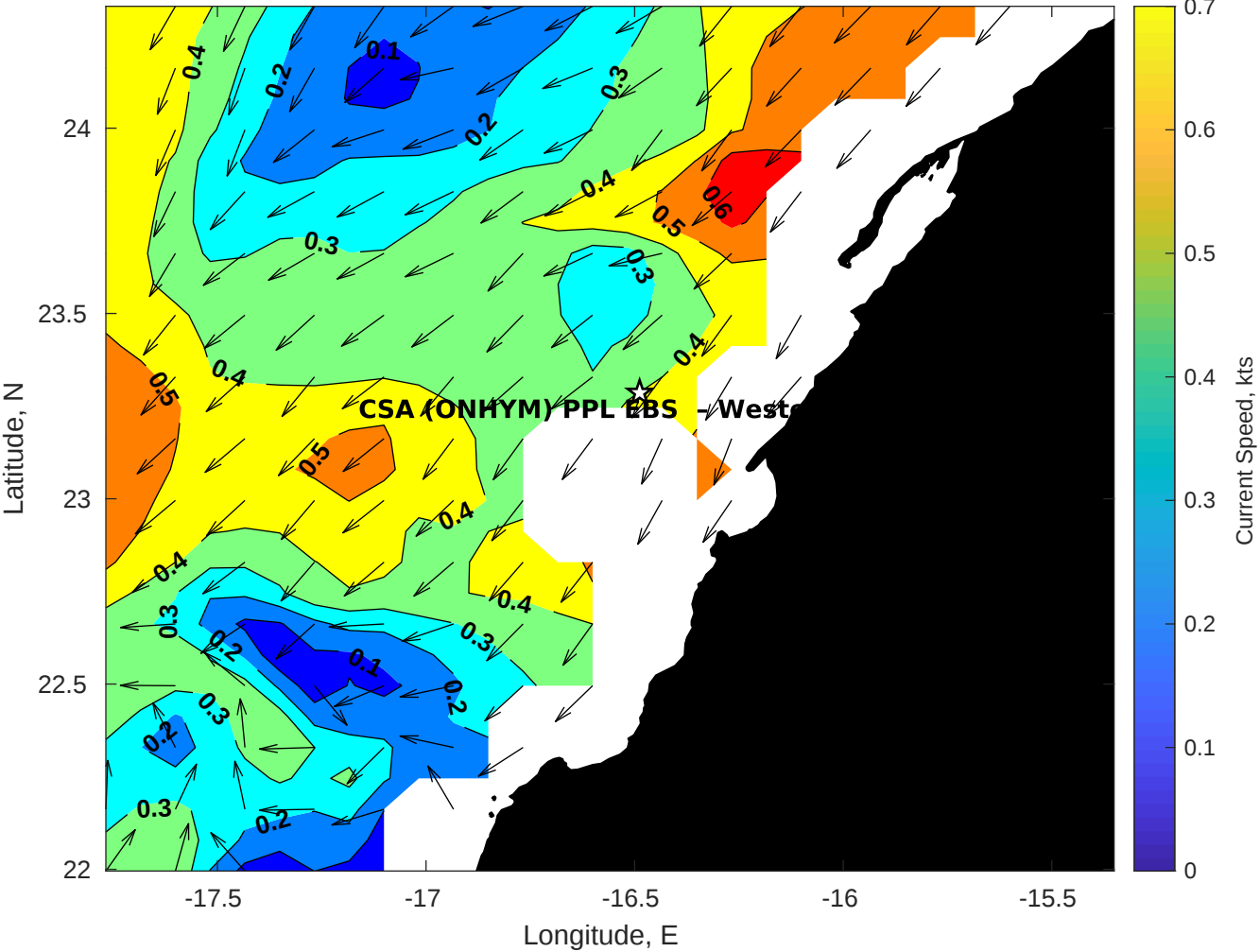
Surface Currents for CSA (ONHYM) PPL EBS - Western Sahara at 30-Aug-2025 00:00:00
