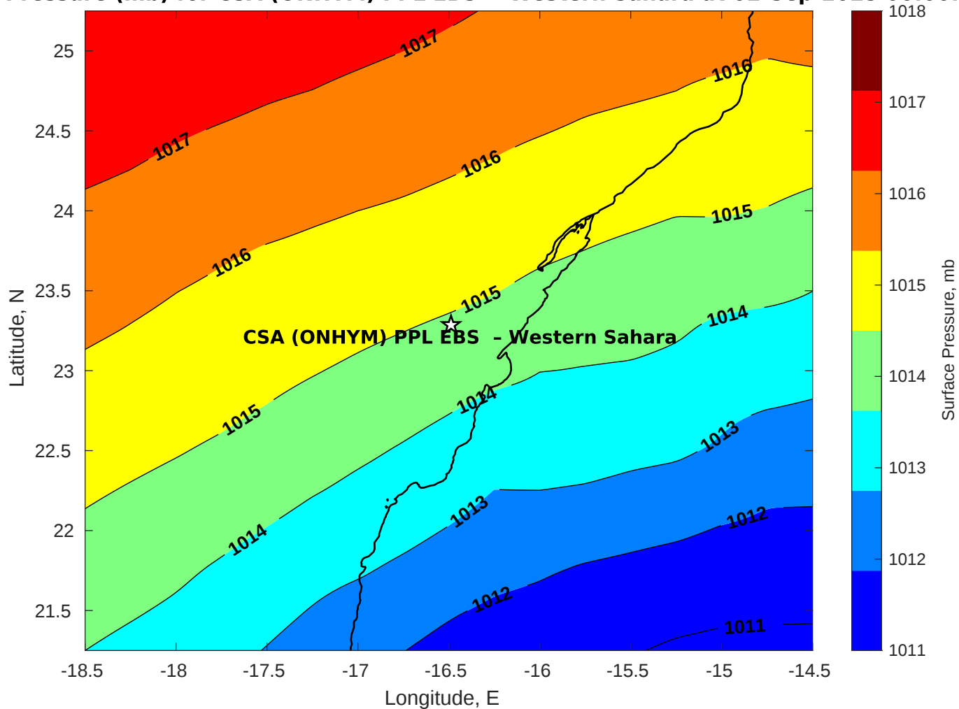
Surface Pressure (mb) for CSA (ONHYM) PPL EBS - Western Sahara at 02-Sep-2025 00:00:00
