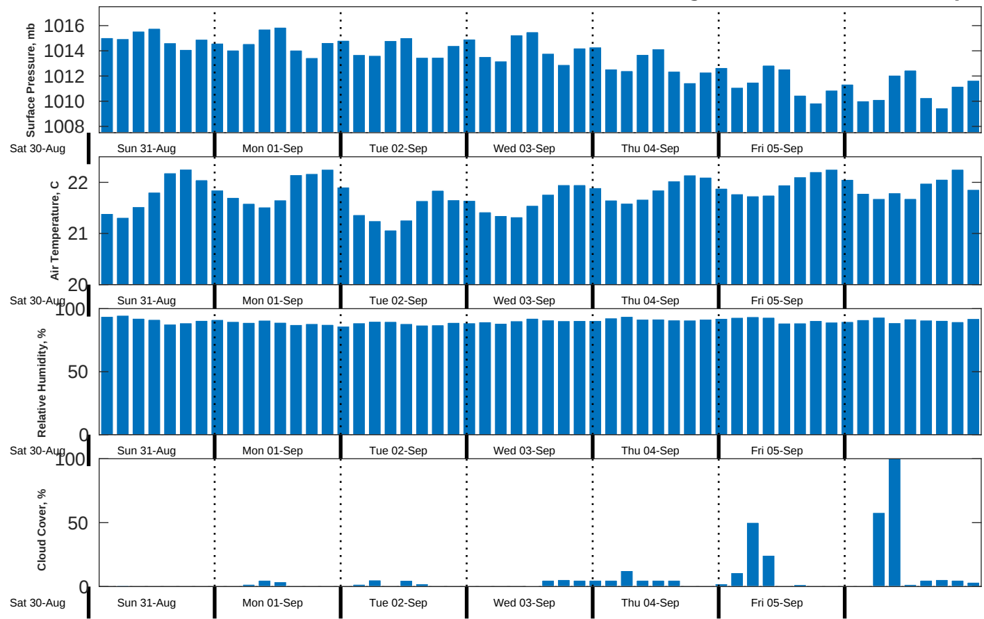
Met Forecast for CSA (ONHYM) PPL EBS - Western Sahara from 31-Aug-2025 00:00:00 to 07-Sep-2025 00:00:00
