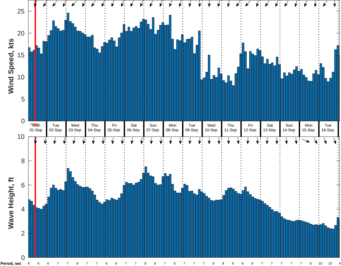
Wind & Wave Forecast for CSA (ONHYM) PPL EBS - Western Sahara from 31-Aug-2025 01:00:00 to 16-Sep-2025 01:00:00
