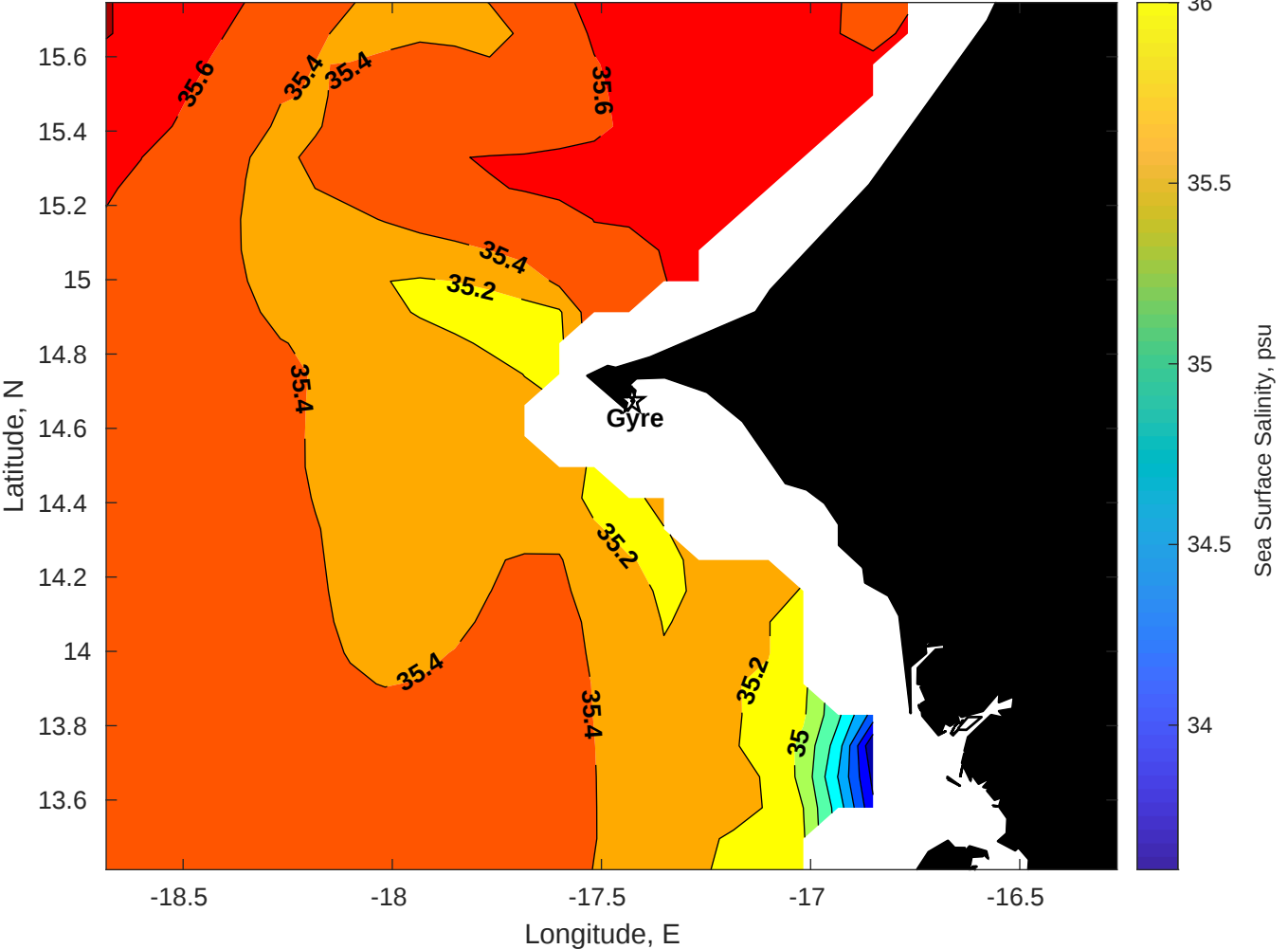
Surface Salinity for Gyre at 30-Aug-2025 00:00:00
