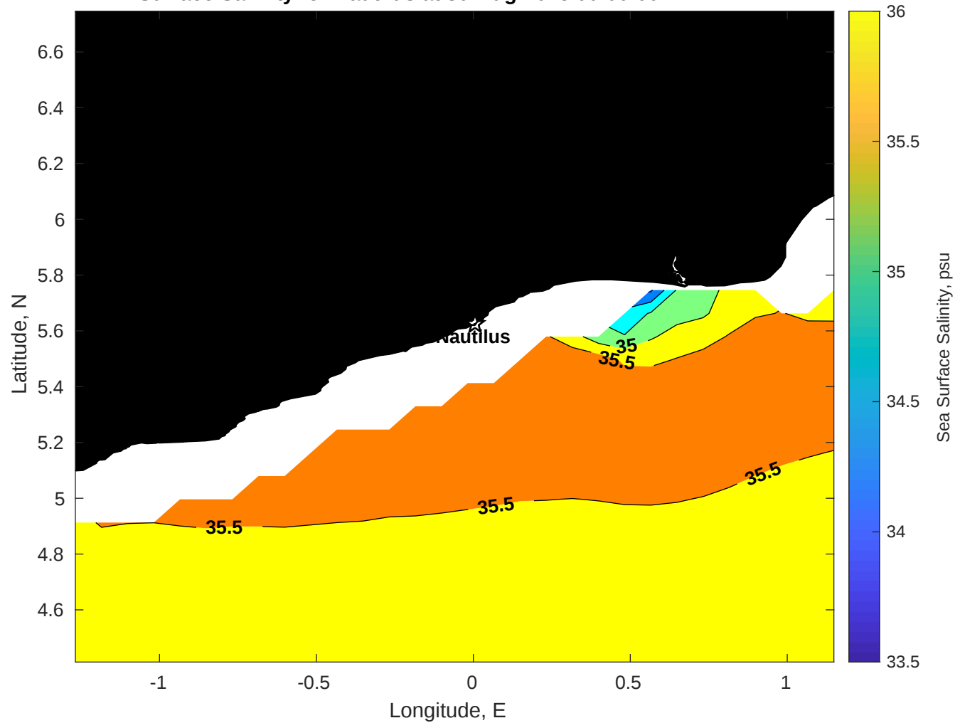
Surface Salinity for Nautilus at 30-Aug-2025 00:00:00
