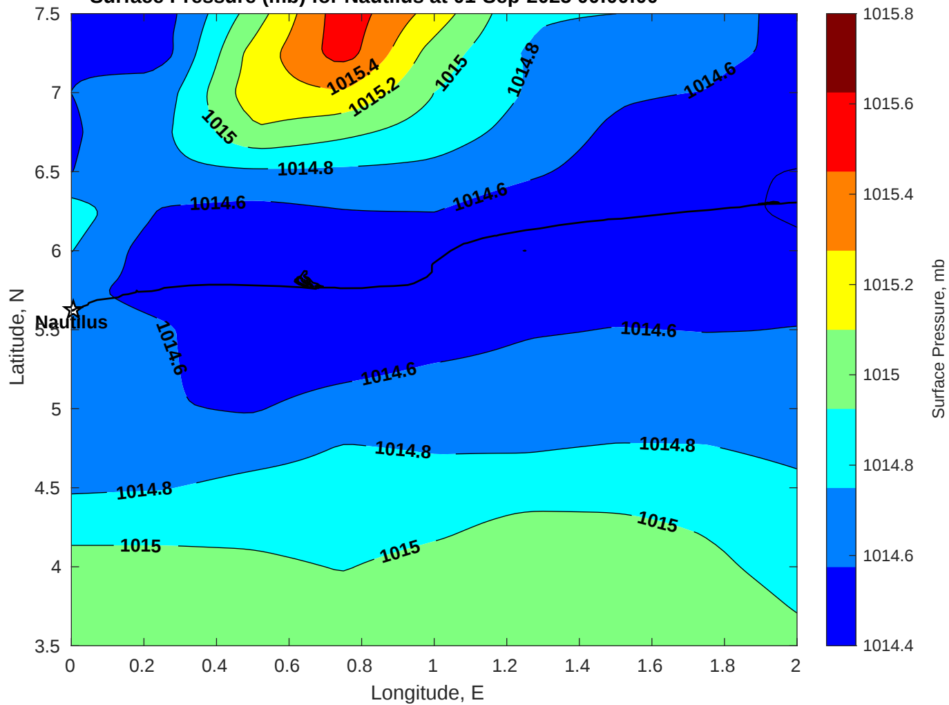
Surface Pressure (mb) for Nautilus at 01-Sep-2025 00:00:00
