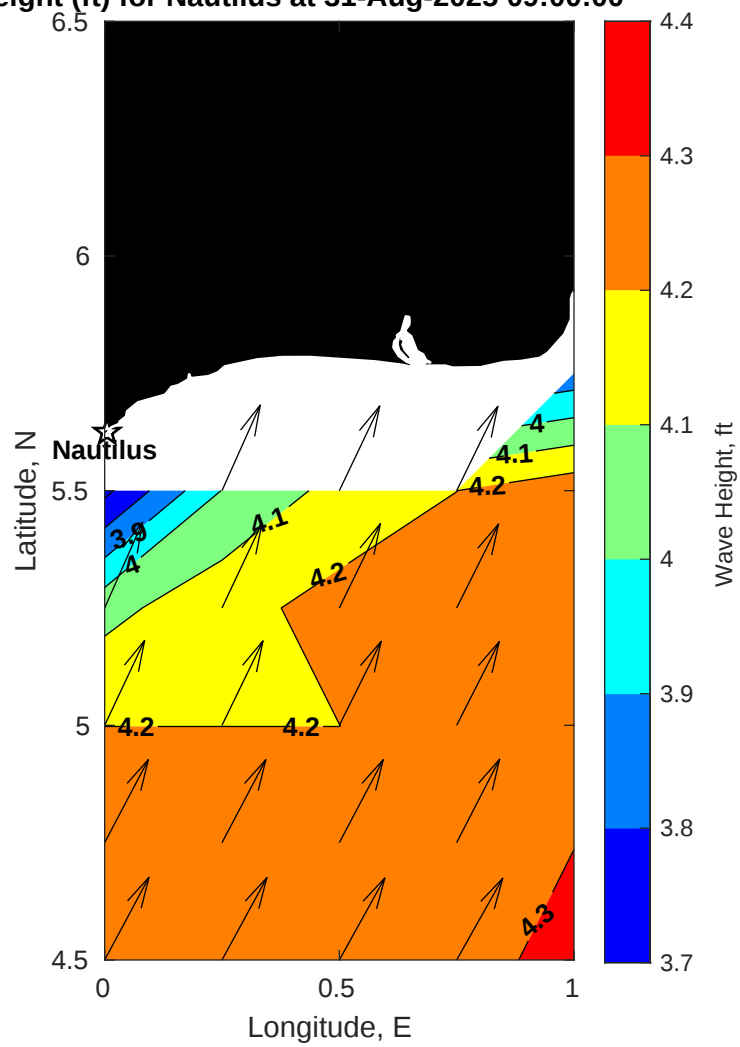
Wave Height (ft) for Nautilus at 31-Aug-2025 09:00:00
