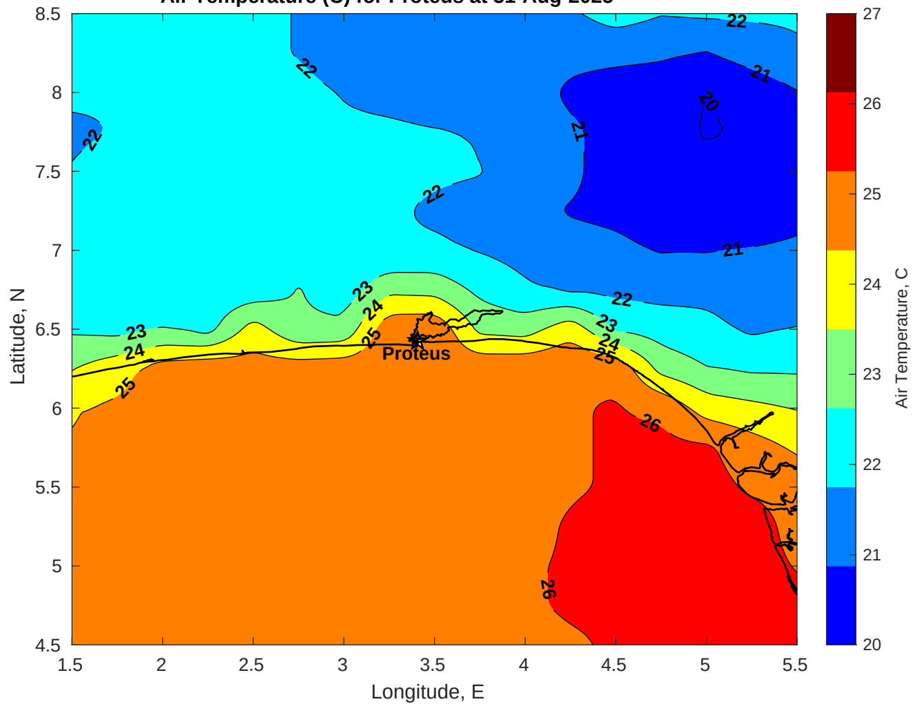
Air Temperature (C) for Proteus at 31-Aug-2025
