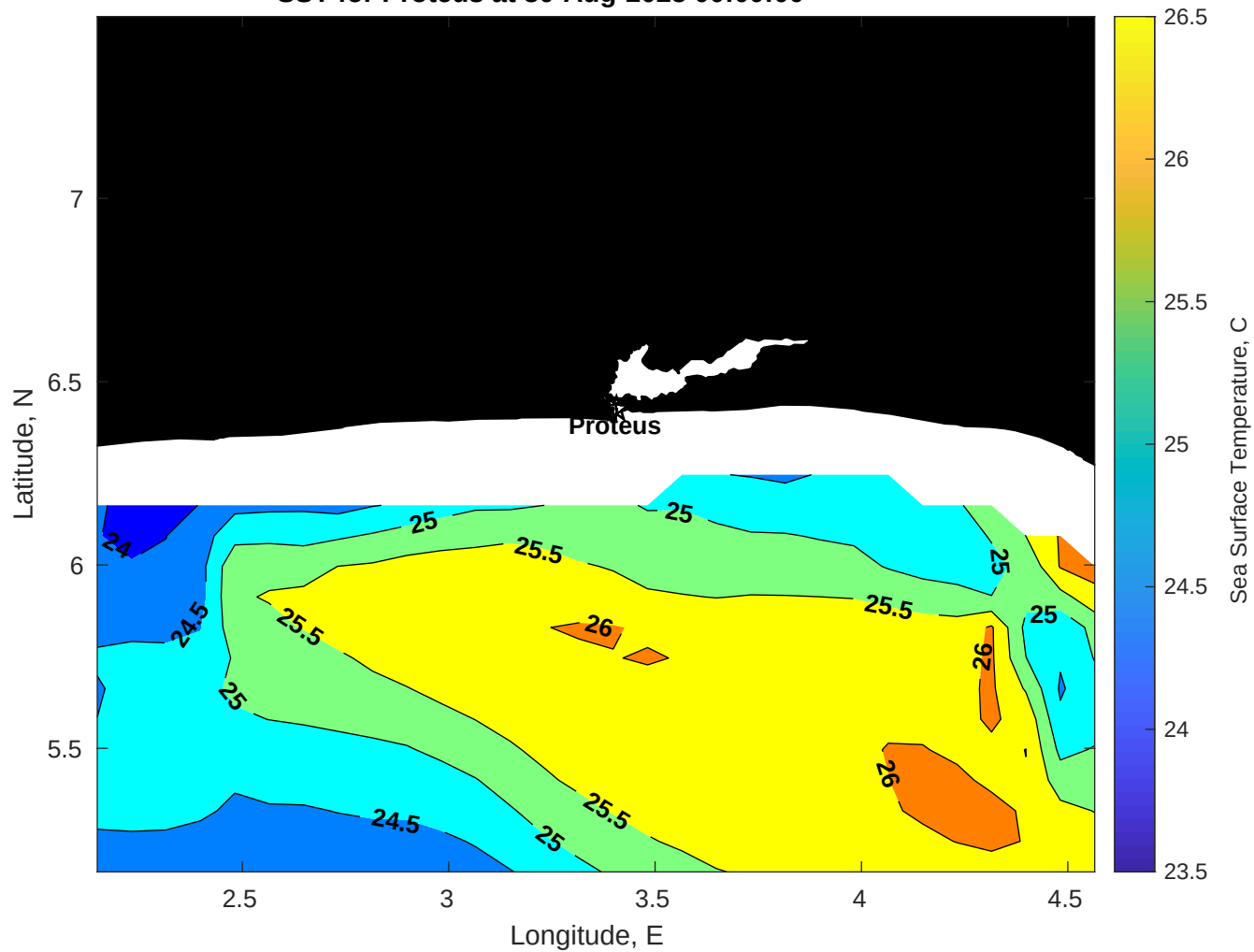
SST for Proteus at 30-Aug-2025 00:00:00
